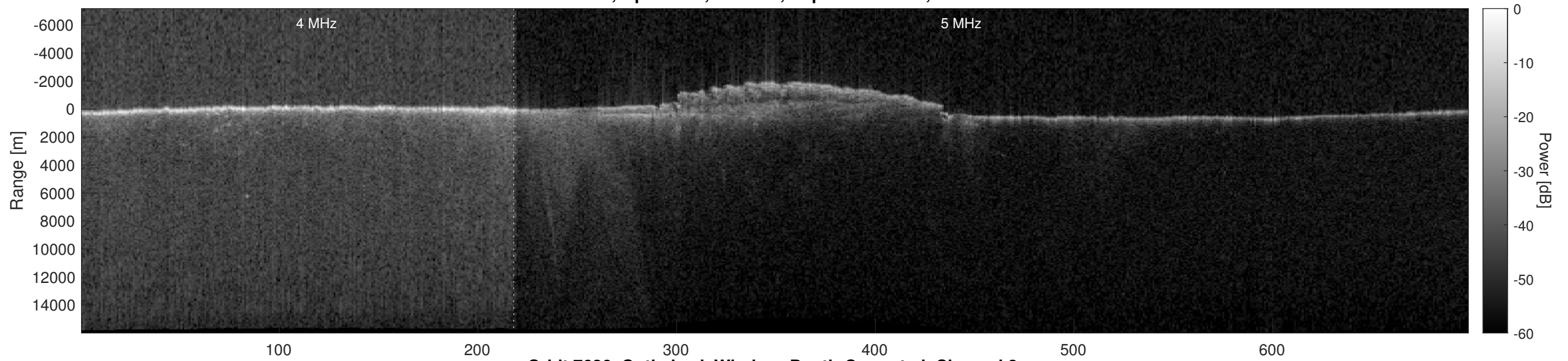
Orbit 7626, Optimized, Window, Depth-Corrected, Channel 2
