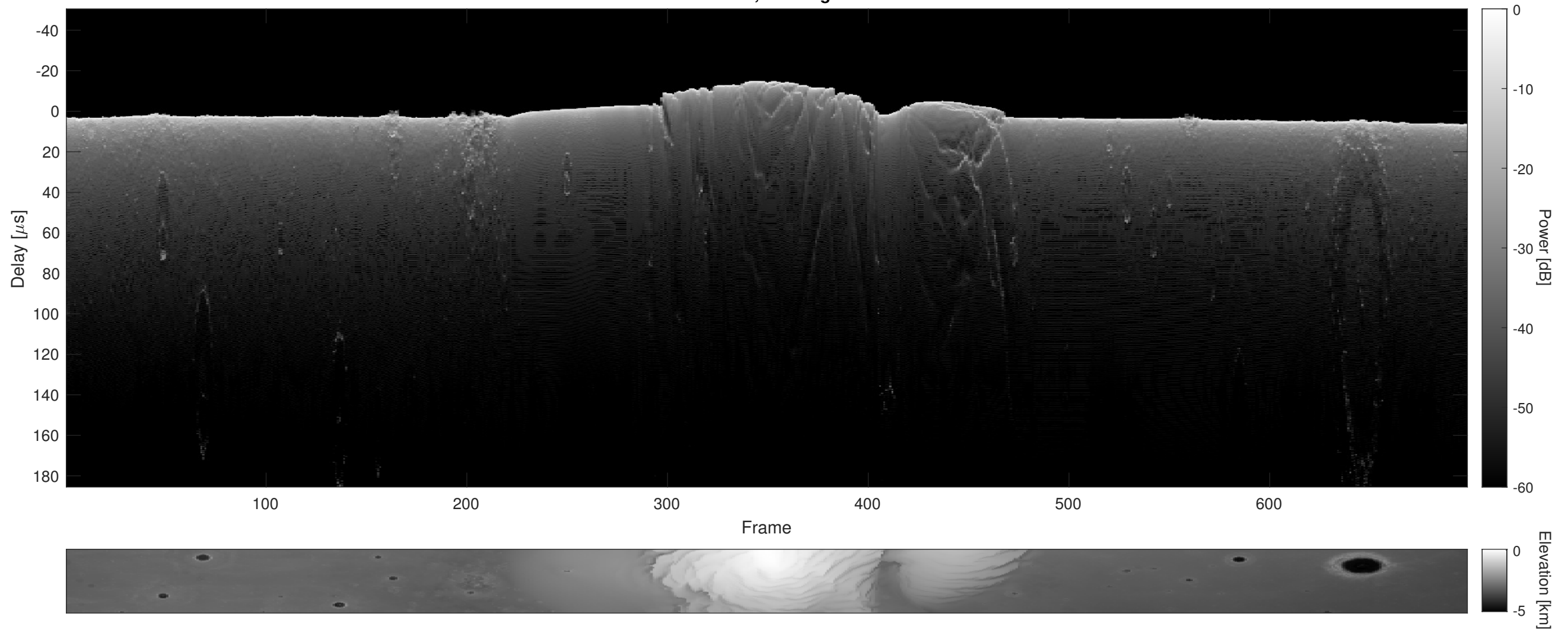
Orbit 7629, Cluttergram
