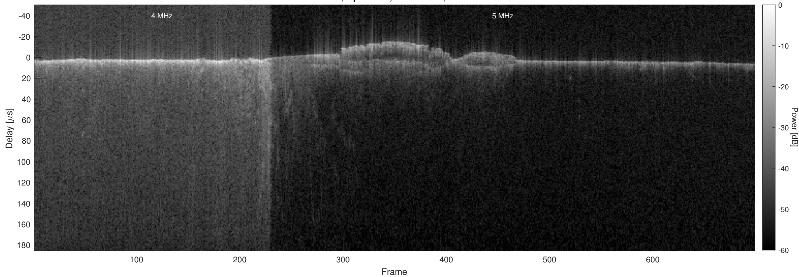
Orbit 7629, Optimized, No Window, Channel 2
