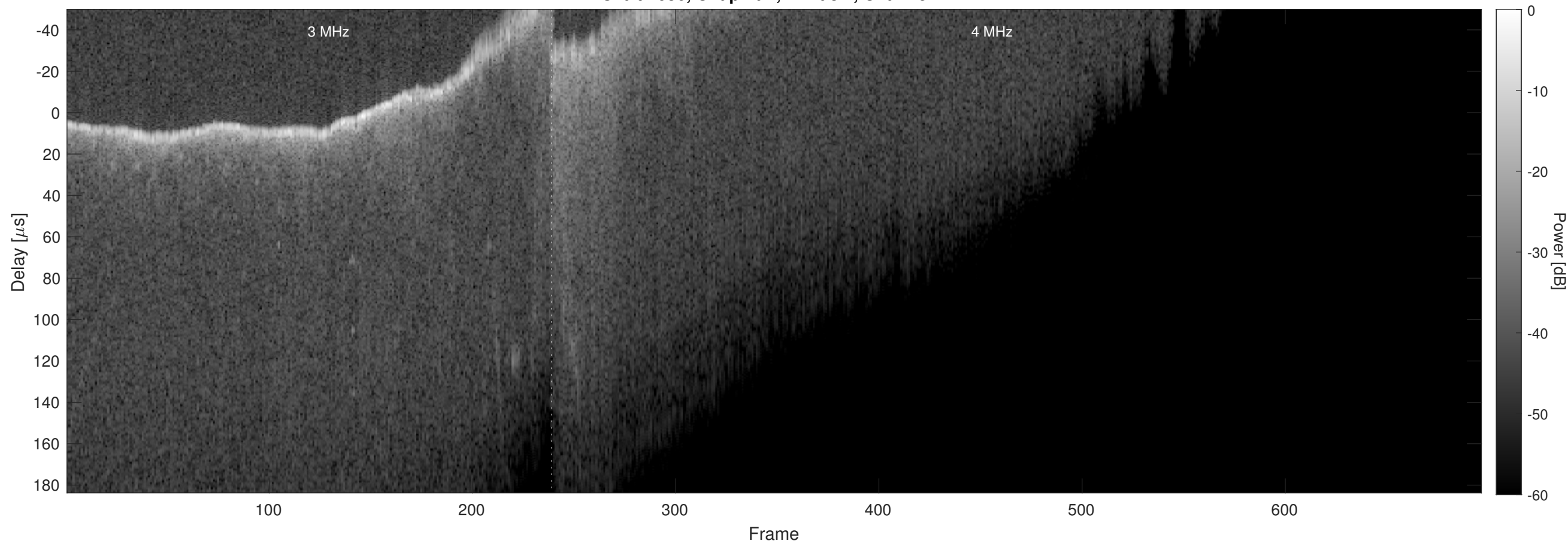
Orbit 7636, Chapman, Window, Channel 2
