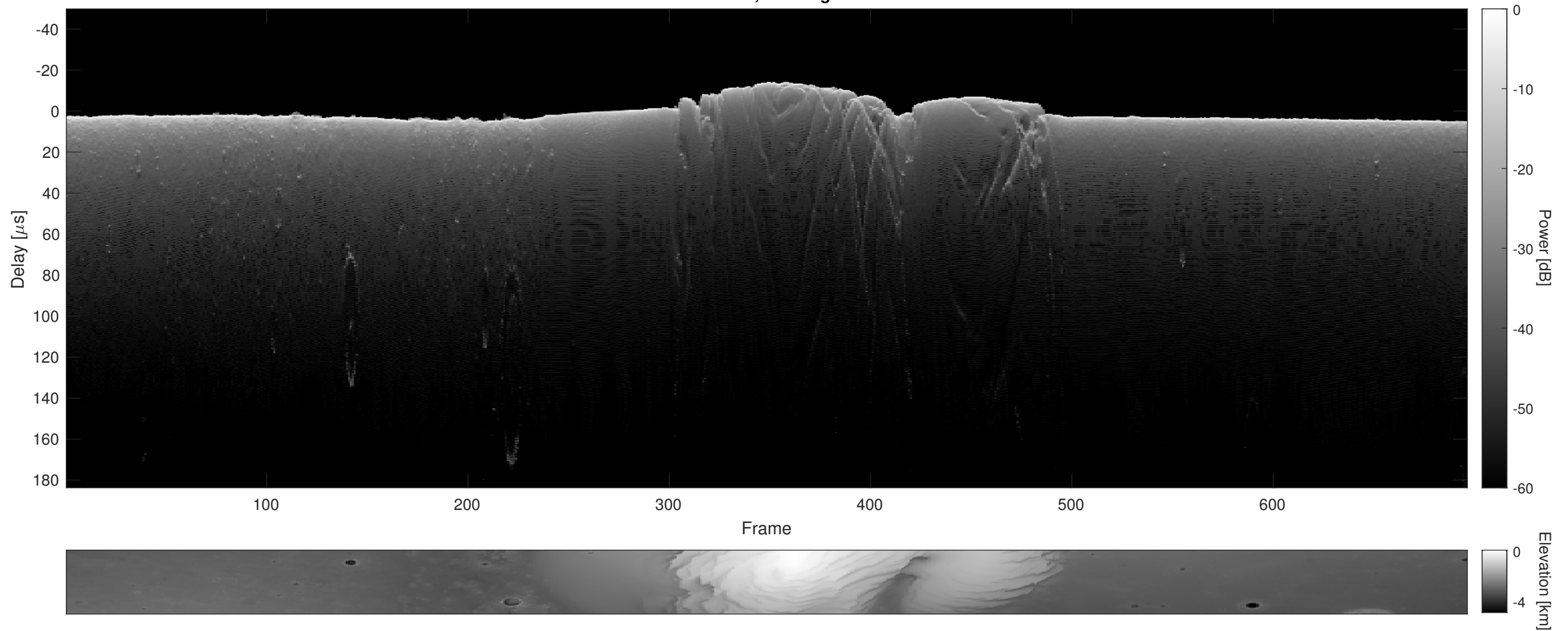
Orbit 7636, Cluttergram
