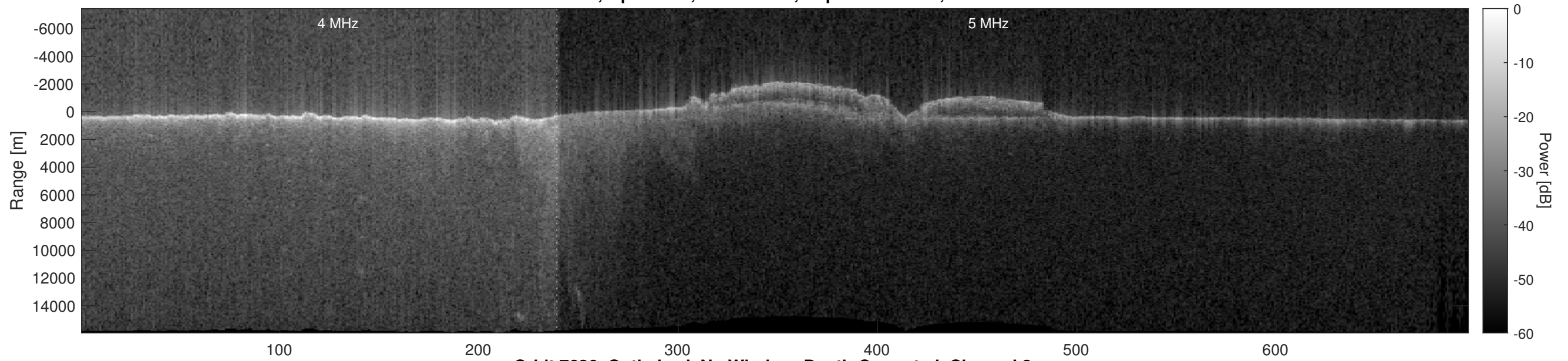
Orbit 7636, Optimized, No Window, Depth-Corrected, Channel 2
