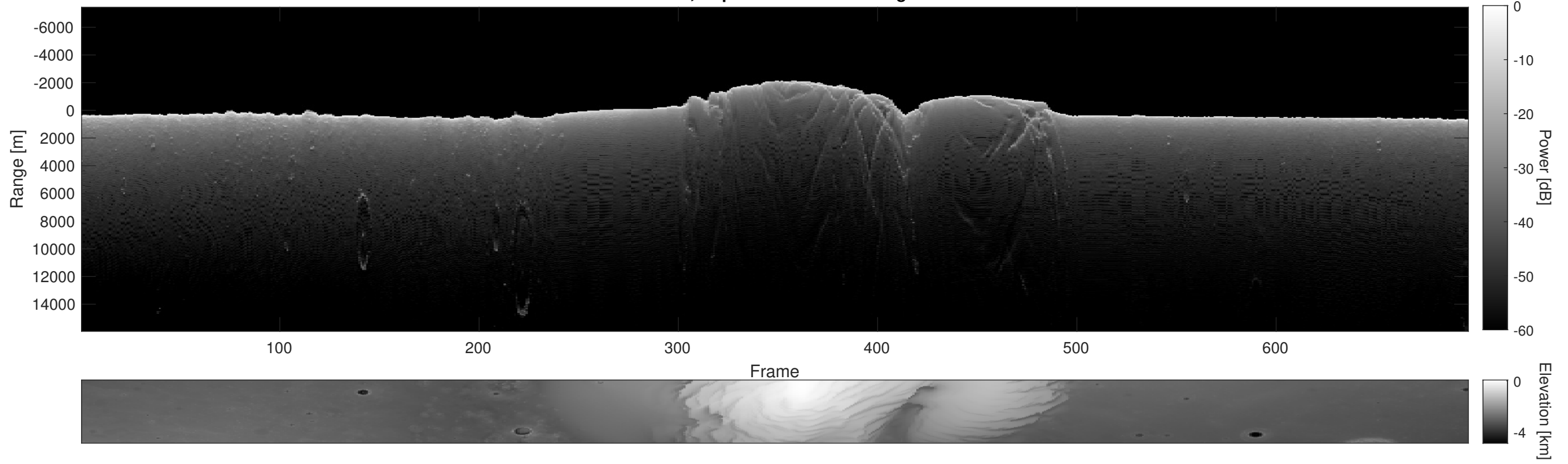
Orbit 7636, Depth-Corrected Cluttergram
