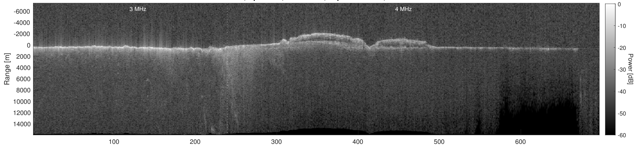
Orbit 7636, Depth-Corrected Cluttergram
