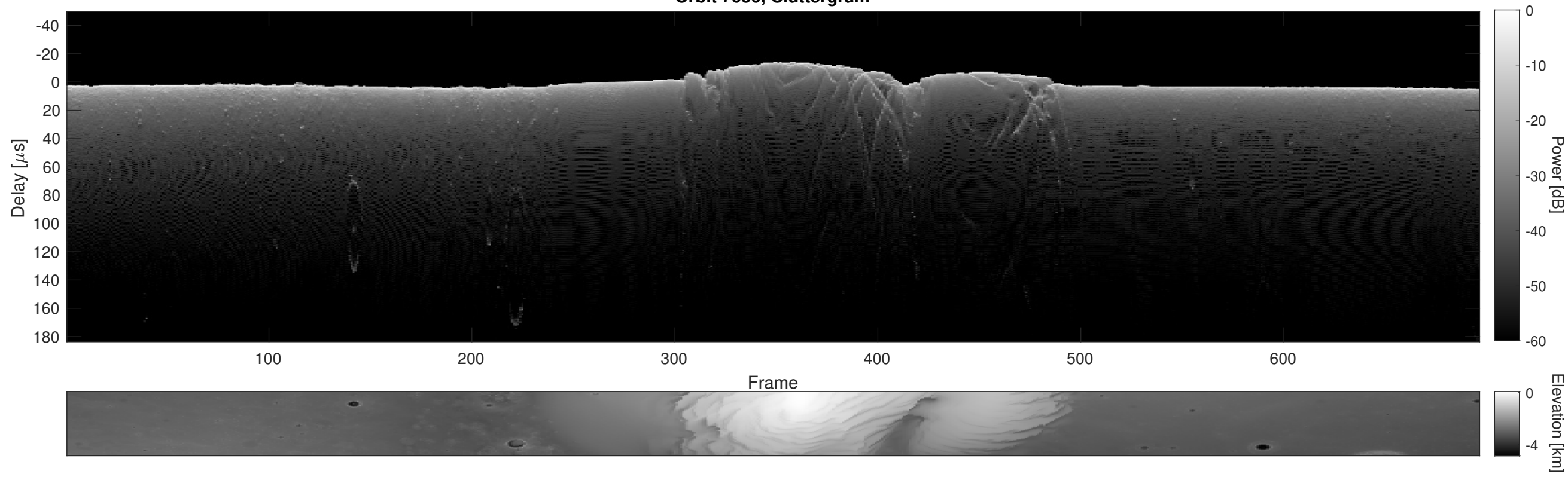
Orbit 7636, Cluttergram
