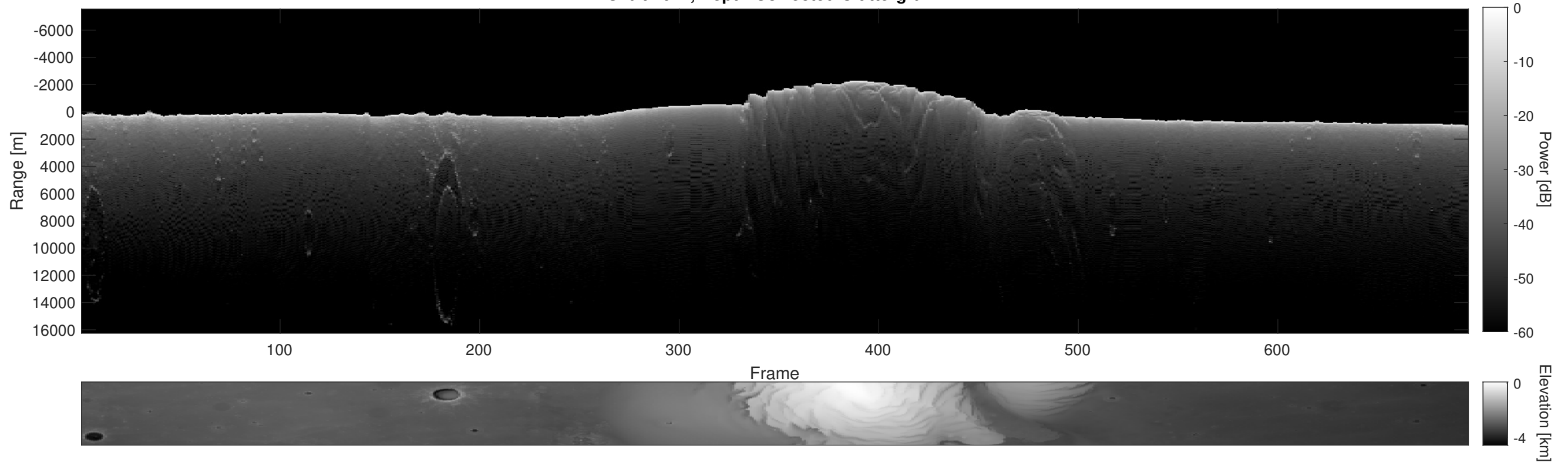
Orbit 7647, Depth-Corrected Cluttergram
