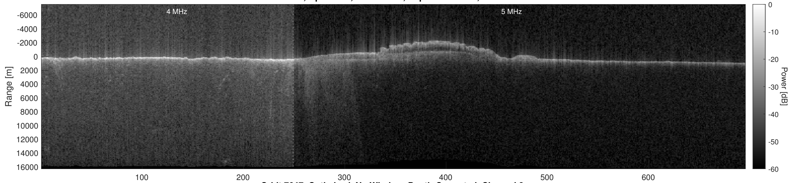
Orbit 7647, Optimized, No Window, Depth-Corrected, Channel 2
