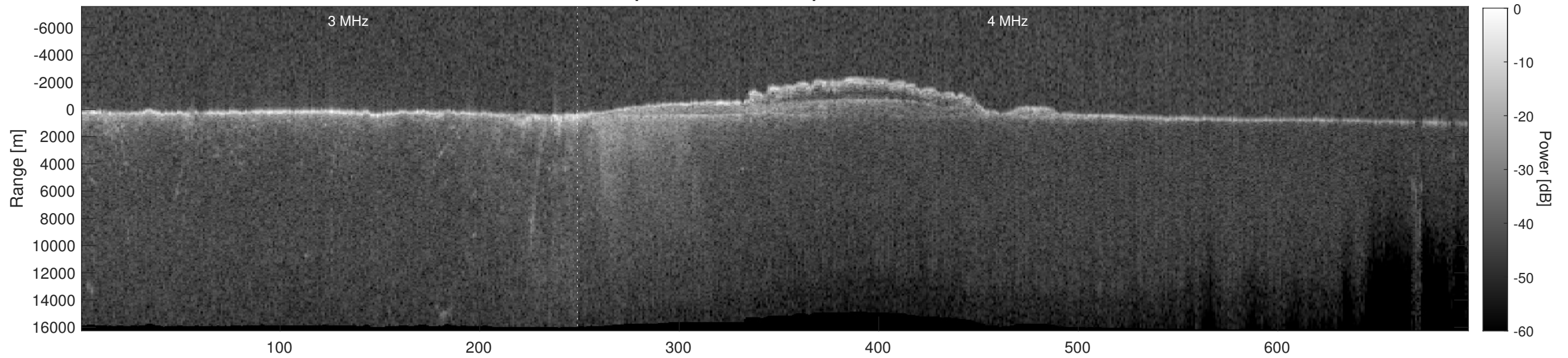
Orbit 7647, Depth-Corrected Cluttergram
