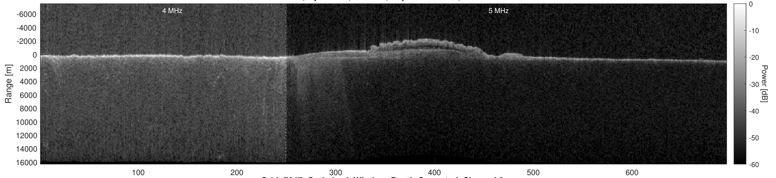
Orbit 7647, Optimized, Window, Depth-Corrected, Channel 2
