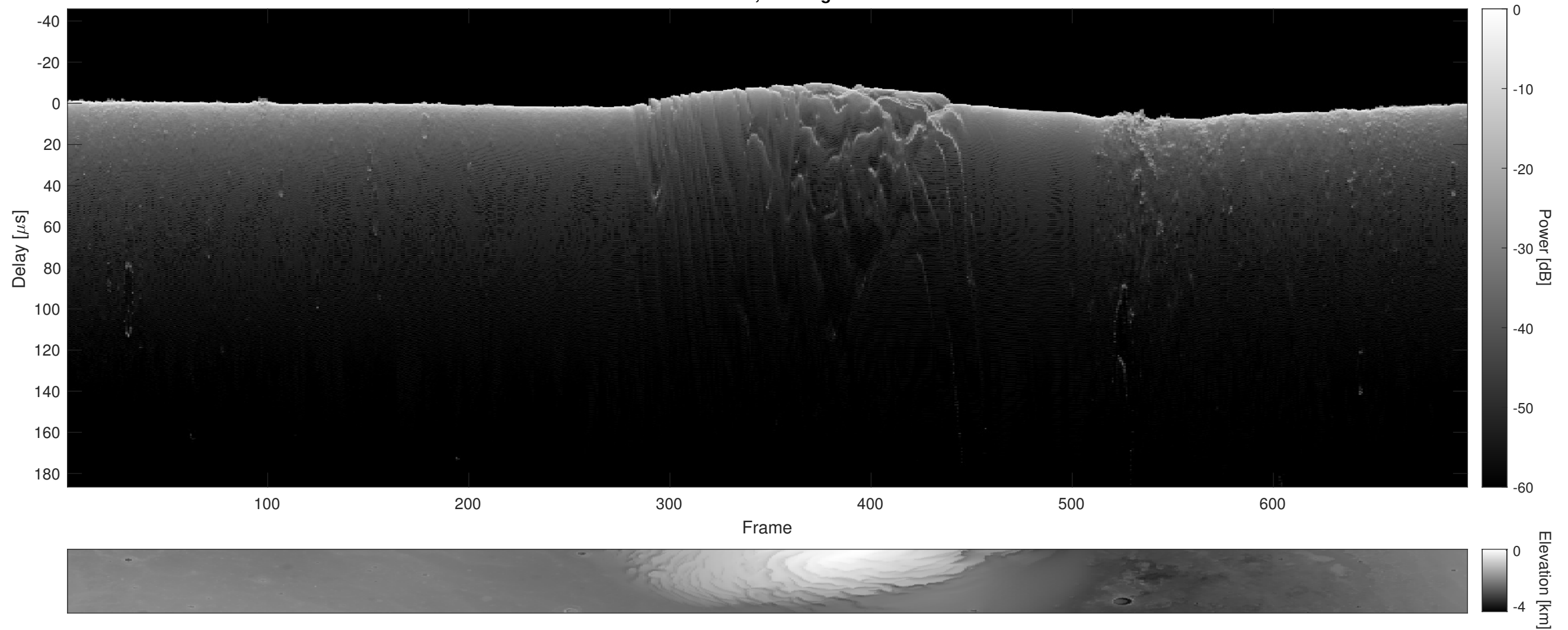
Orbit 7648, Cluttergram
