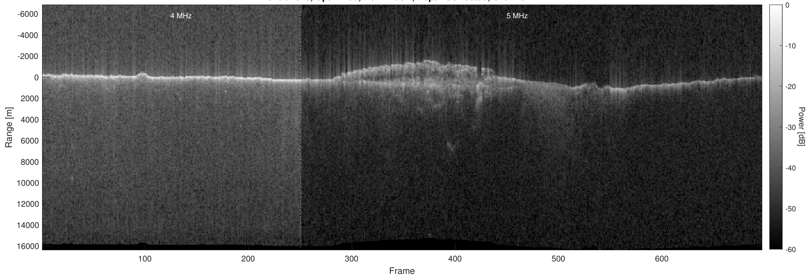
Orbit 7648, Optimized, No Window, Depth-Corrected, Channel 2
