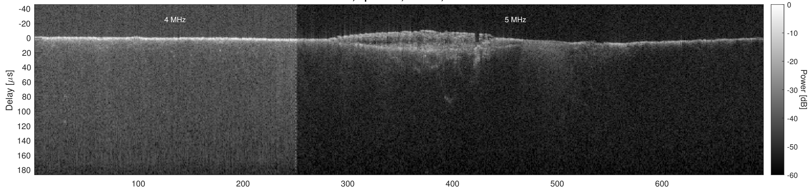
Orbit 7648, Optimized, Window, Channel 2
