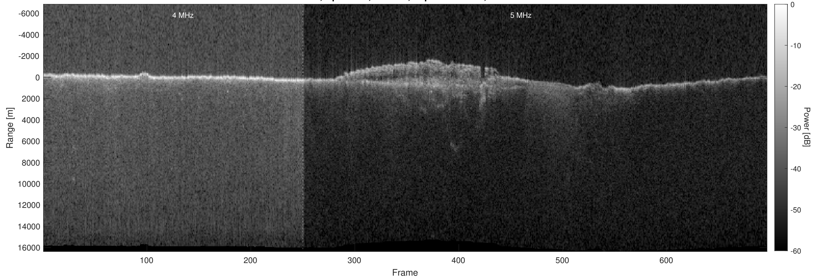
Orbit 7648, Optimized, Window, Depth-Corrected, Channel 2
