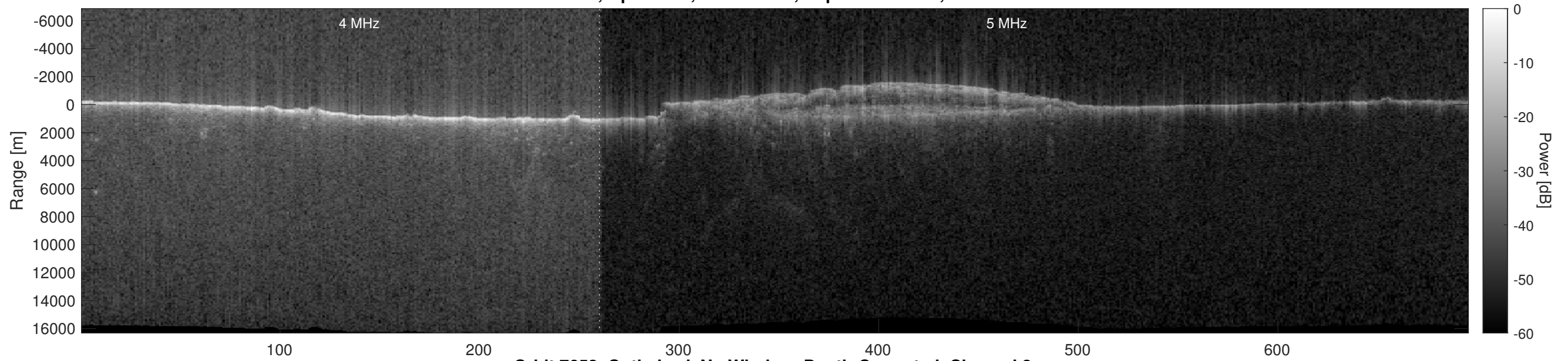
Orbit 7653, Optimized, No Window, Depth-Corrected, Channel 2
