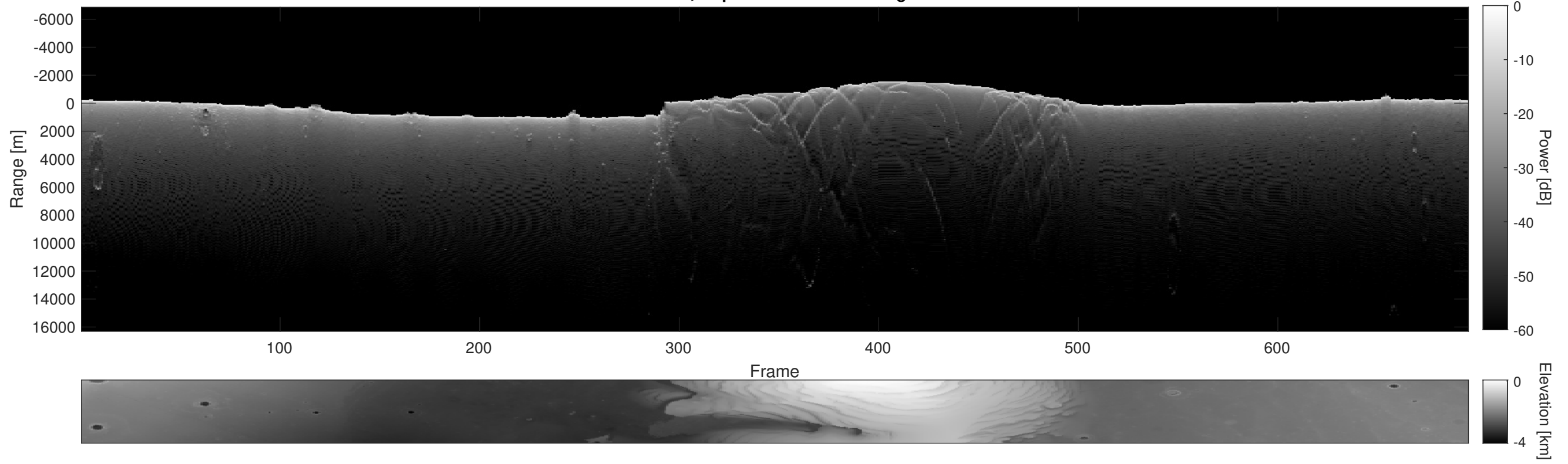
Orbit 7653, Depth-Corrected Cluttergram
