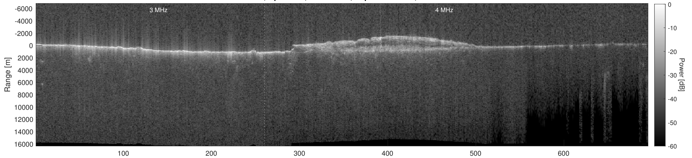
Orbit 7653, Depth-Corrected Cluttergram
