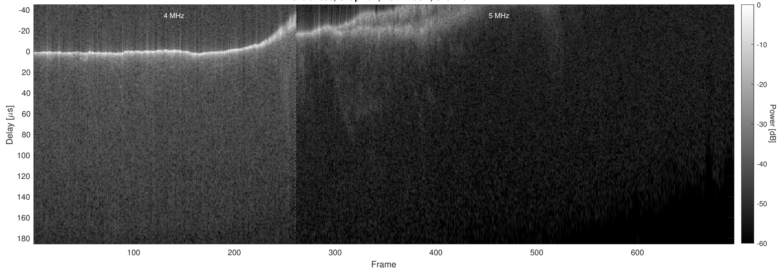
Orbit 7655, Chapman, No Window, Channel 2
