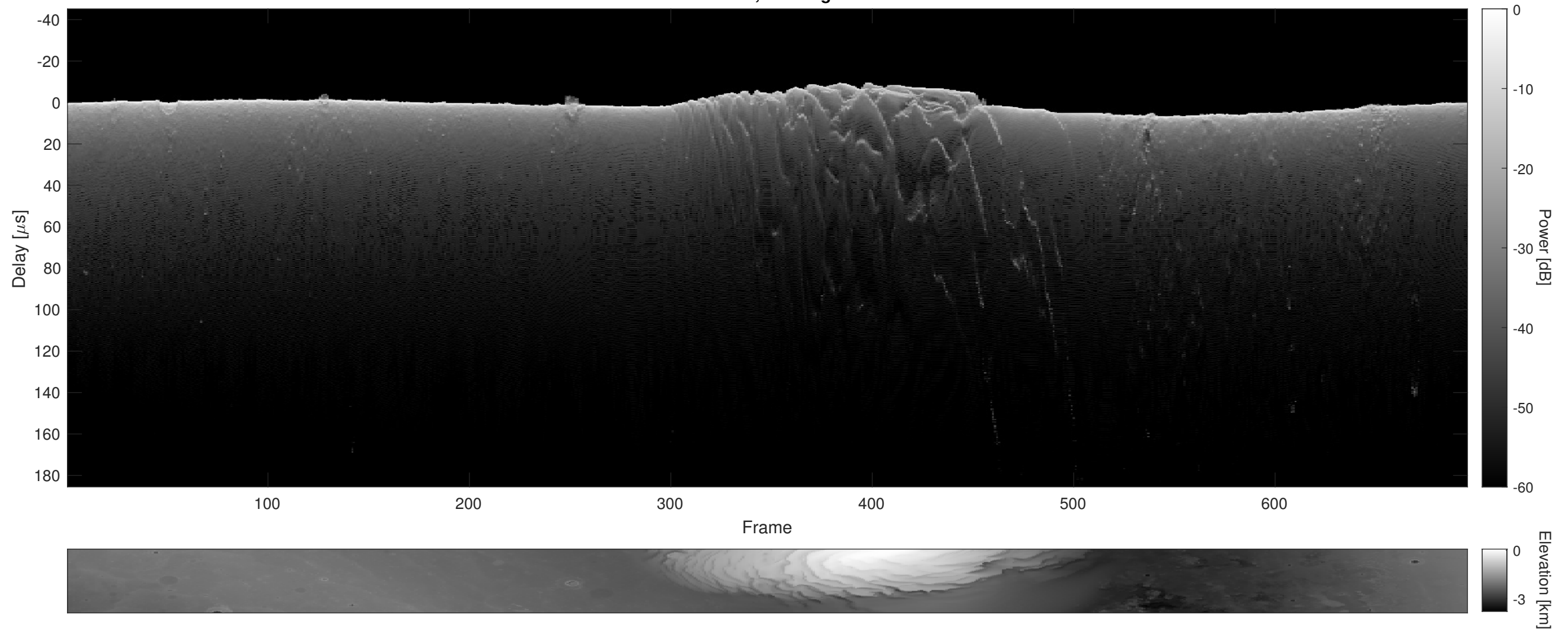
Orbit 7655, Cluttergram
