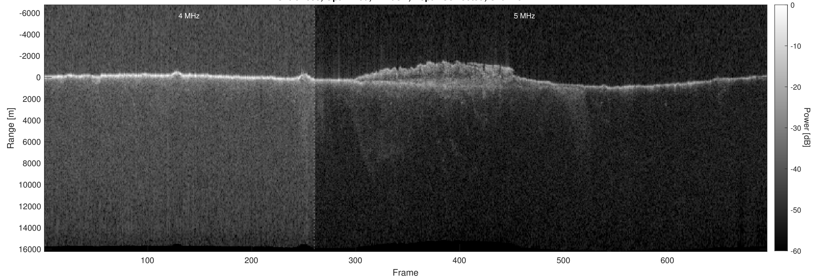
Orbit 7655, Optimized, Window, Depth-Corrected, Channel 2
