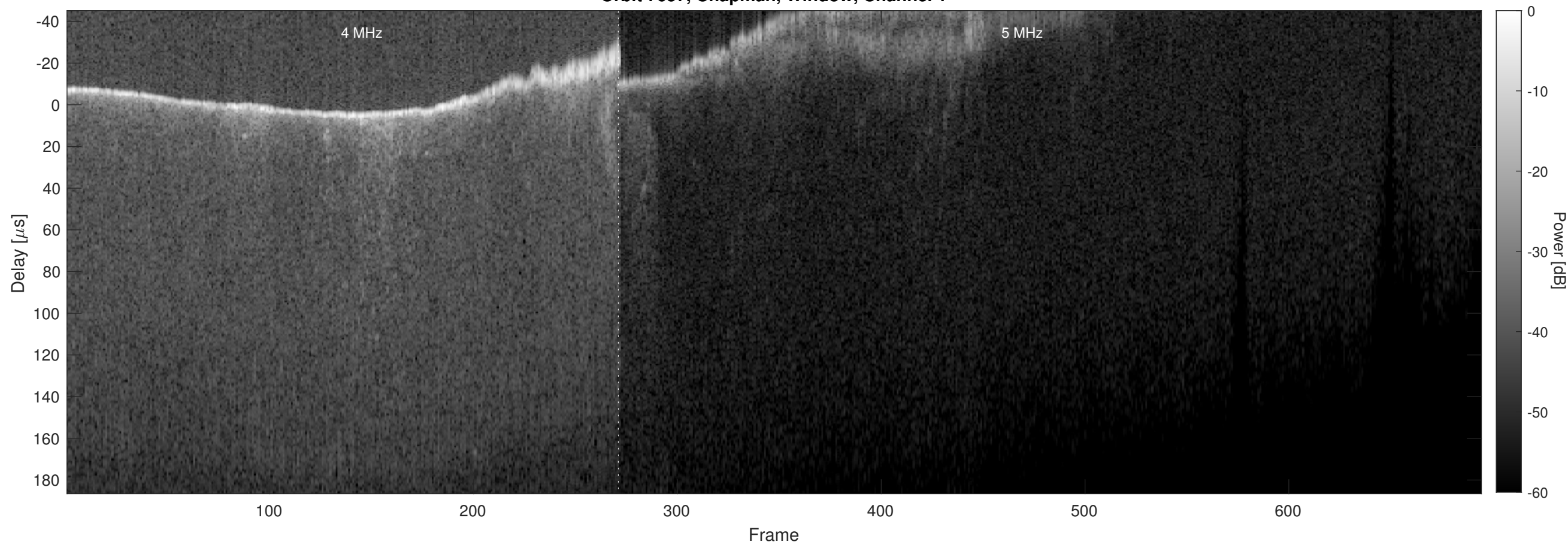
Orbit 7657, Chapman, Window, Channel 2
