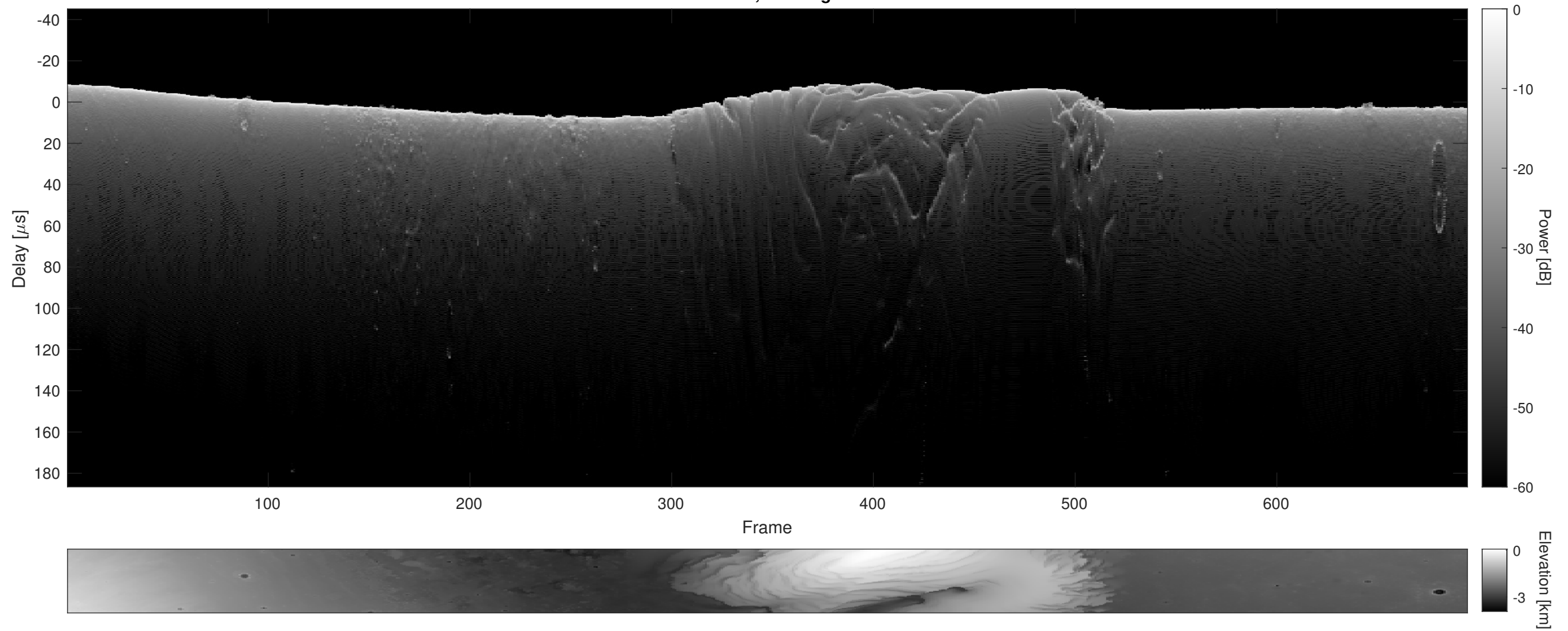
Orbit 7657, Cluttergram
