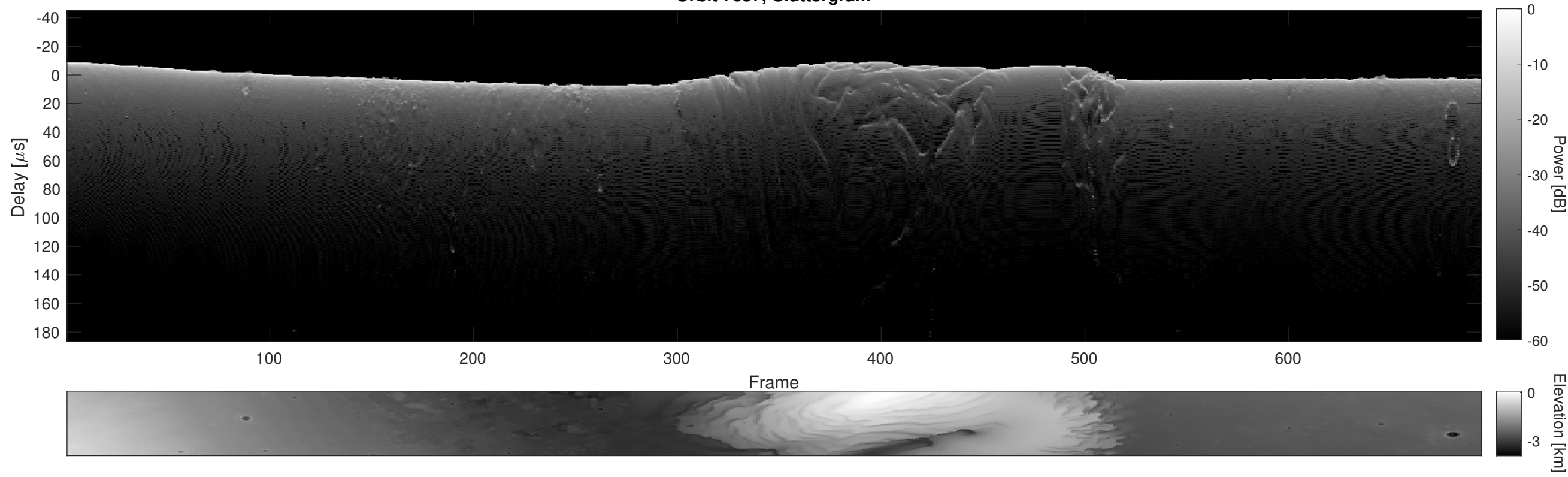
Orbit 7657, Cluttergram
