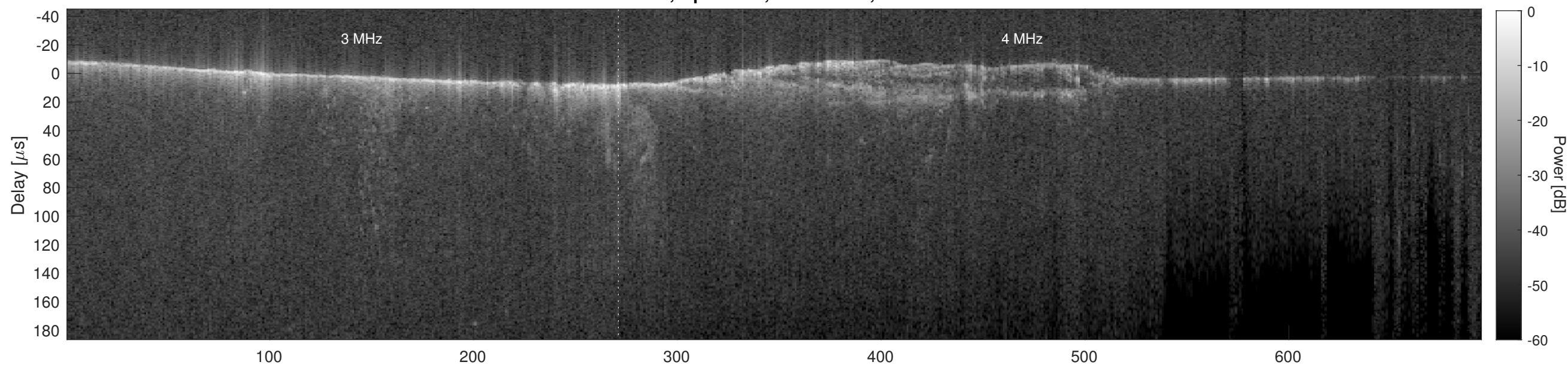
Orbit 7657, Cluttergram
