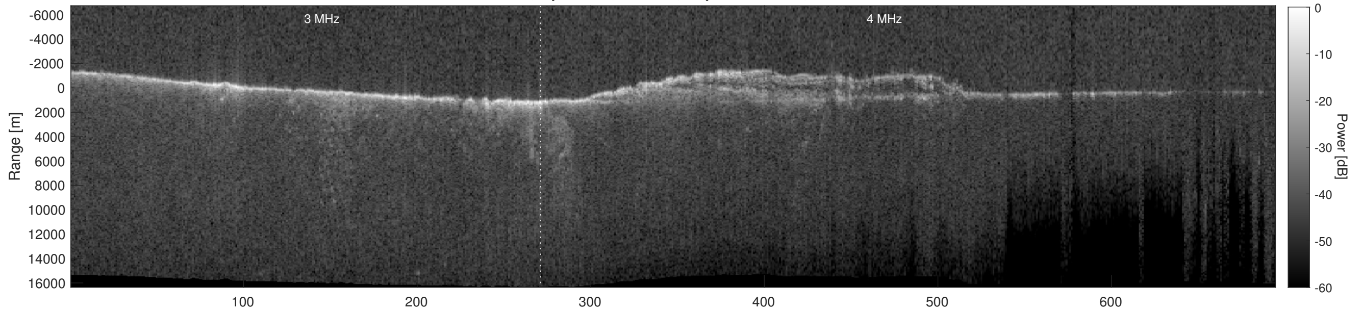
Orbit 7657, Depth-Corrected Cluttergram
