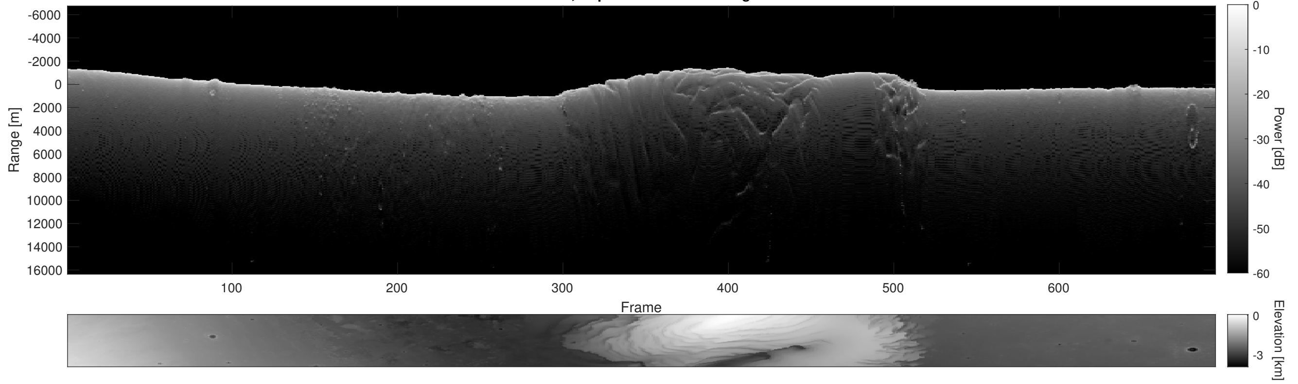
Orbit 7657, Depth-Corrected Cluttergram
