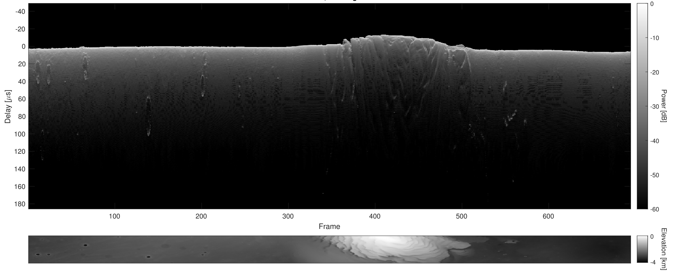
Orbit 7658, Cluttergram
