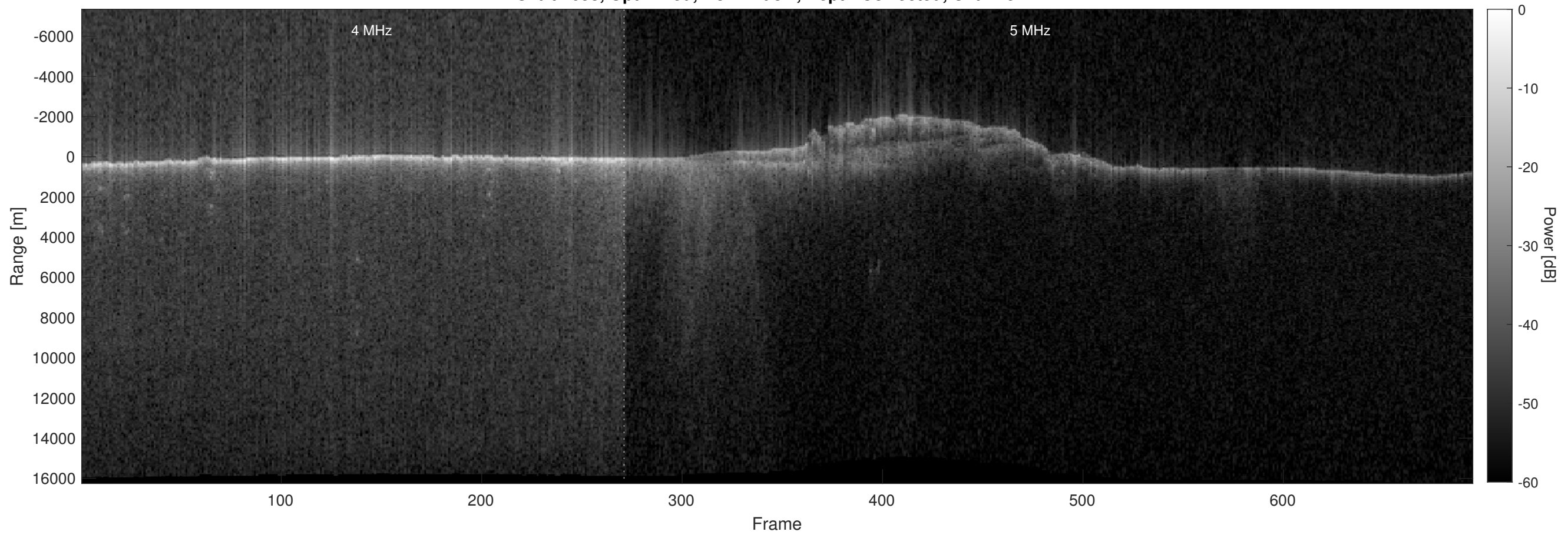
Orbit 7658, Optimized, No Window, Depth-Corrected, Channel 2
