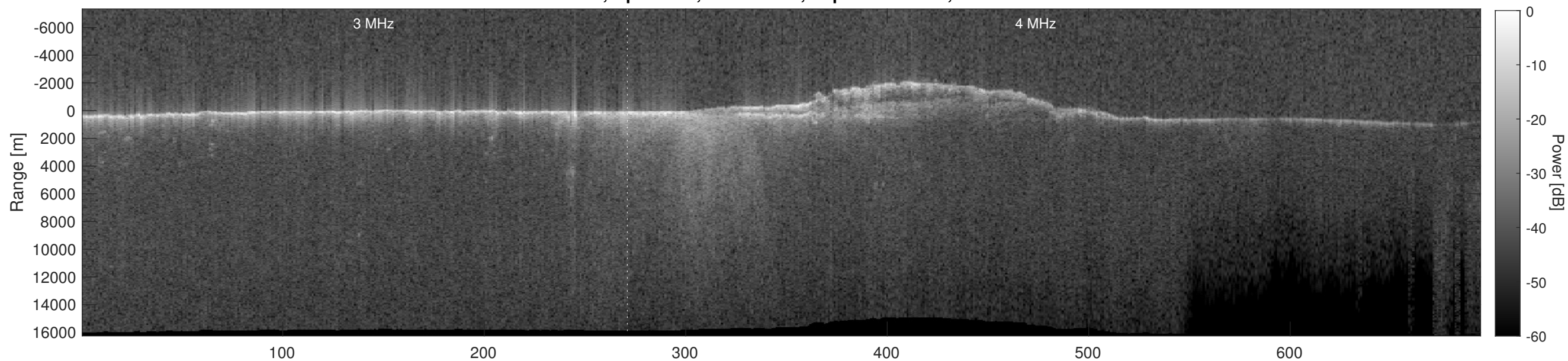
Orbit 7658, Depth-Corrected Cluttergram
