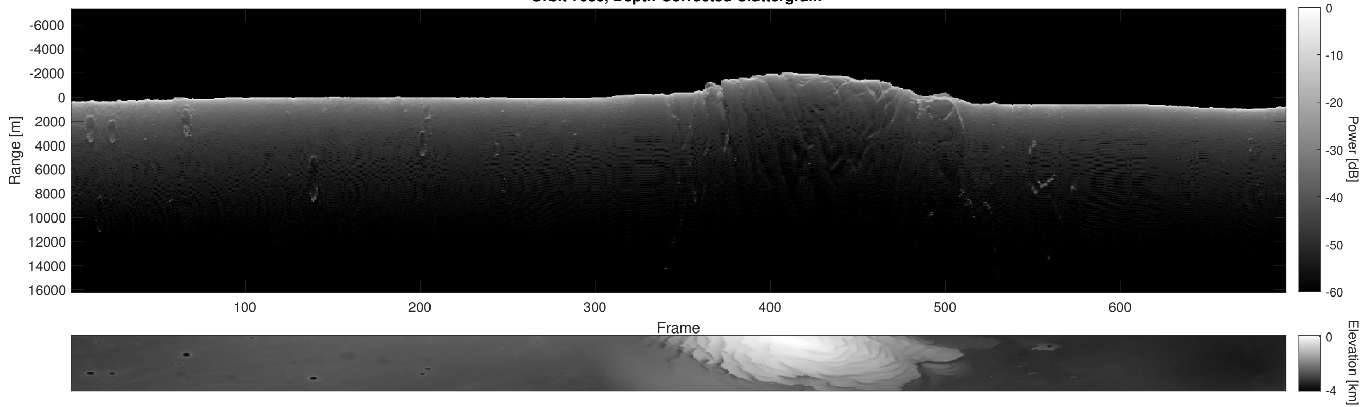
Orbit 7658, Depth-Corrected Cluttergram
