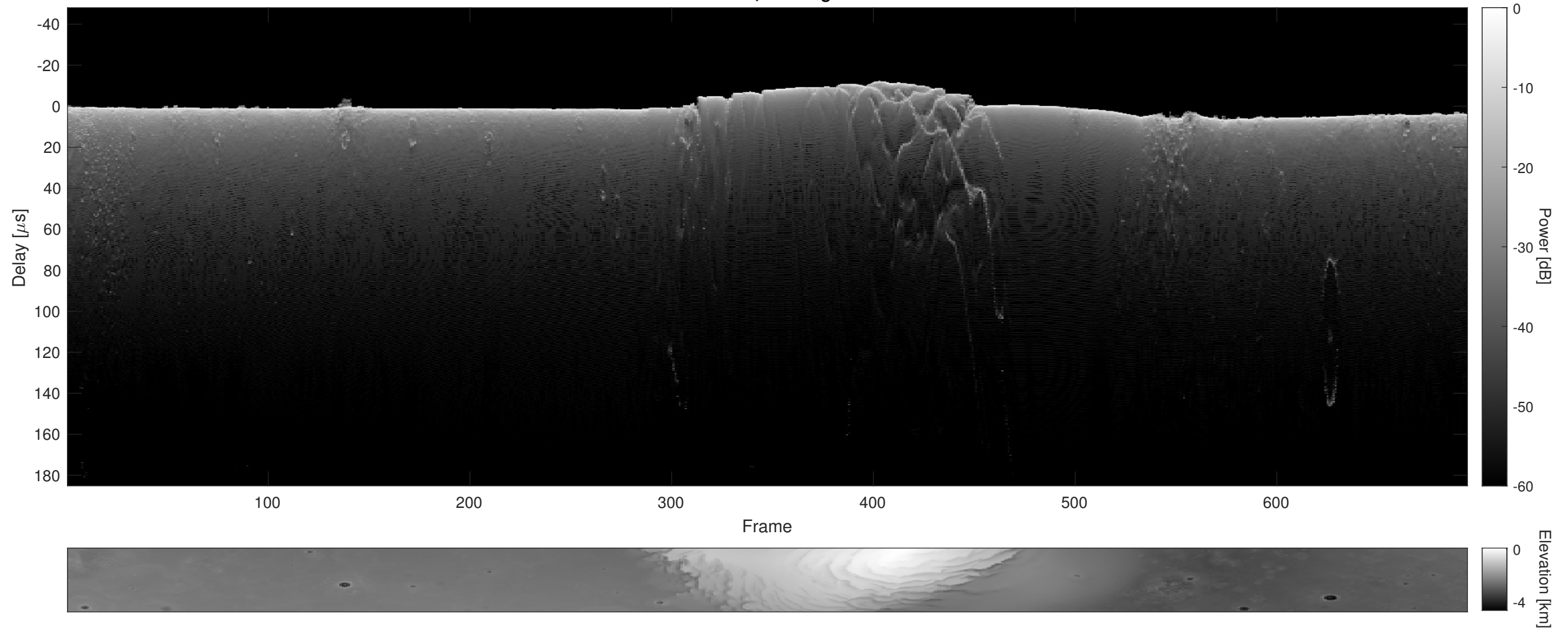
Orbit 7659, Cluttergram
