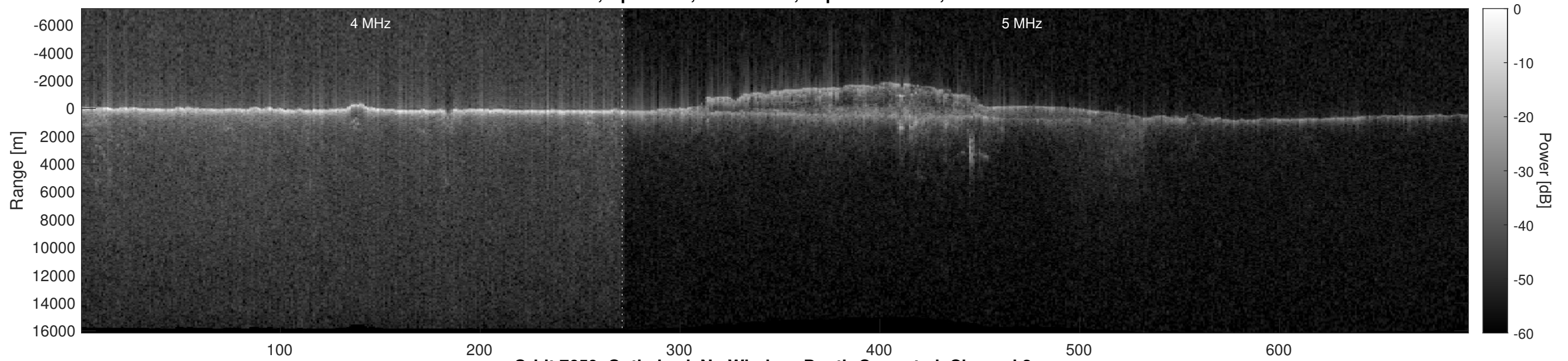
Orbit 7659, Optimized, No Window, Depth-Corrected, Channel 2
