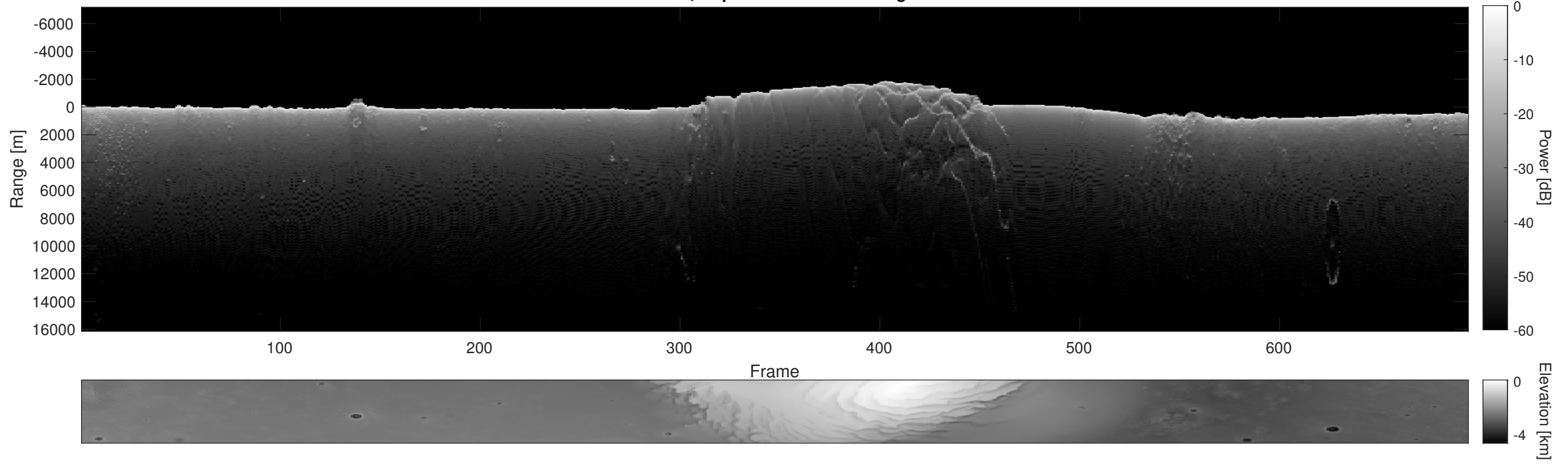
Orbit 7659, Depth-Corrected Cluttergram
