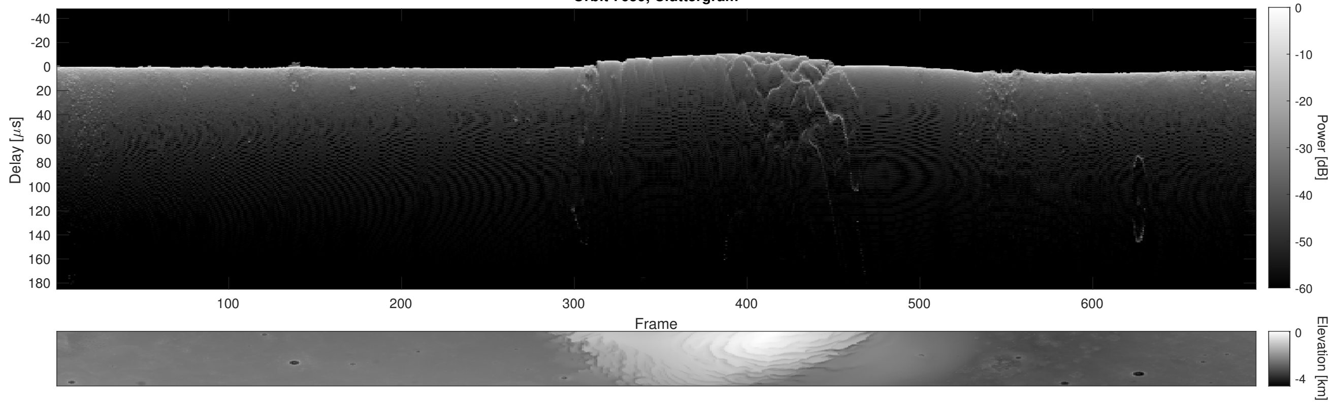
Orbit 7659, Cluttergram
