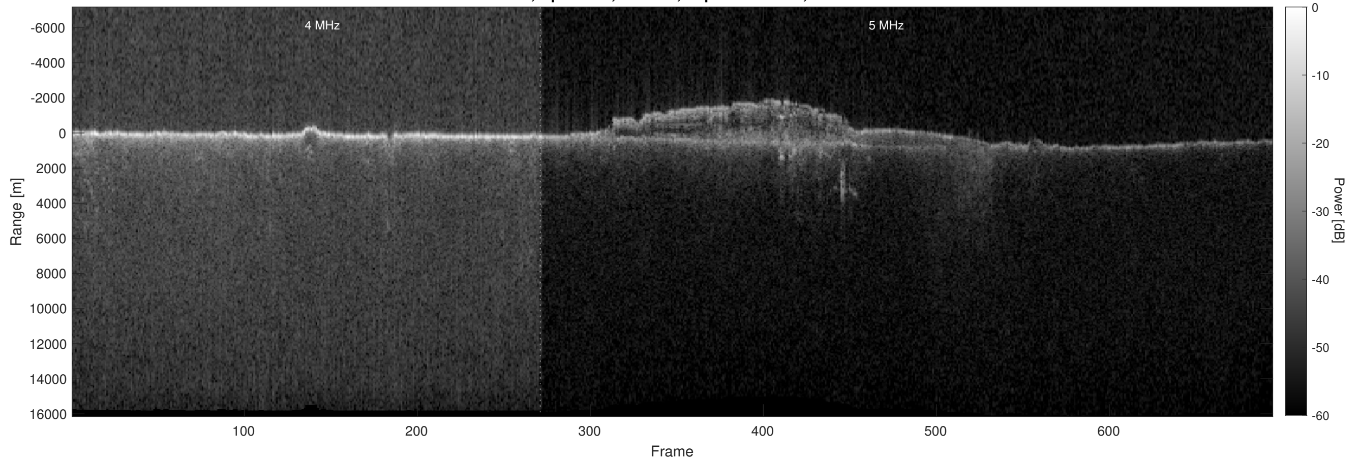
Orbit 7659, Optimized, Window, Depth-Corrected, Channel 2
