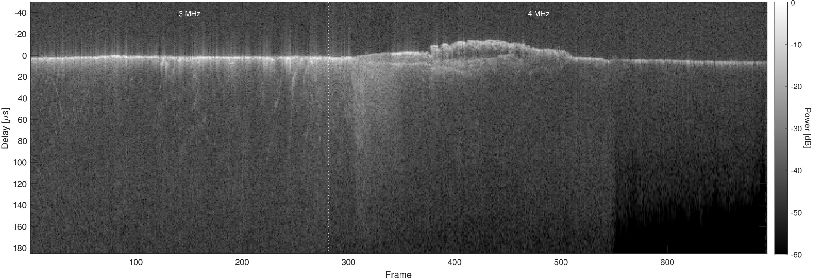
Orbit 7665, Optimized, No Window, Channel 2
