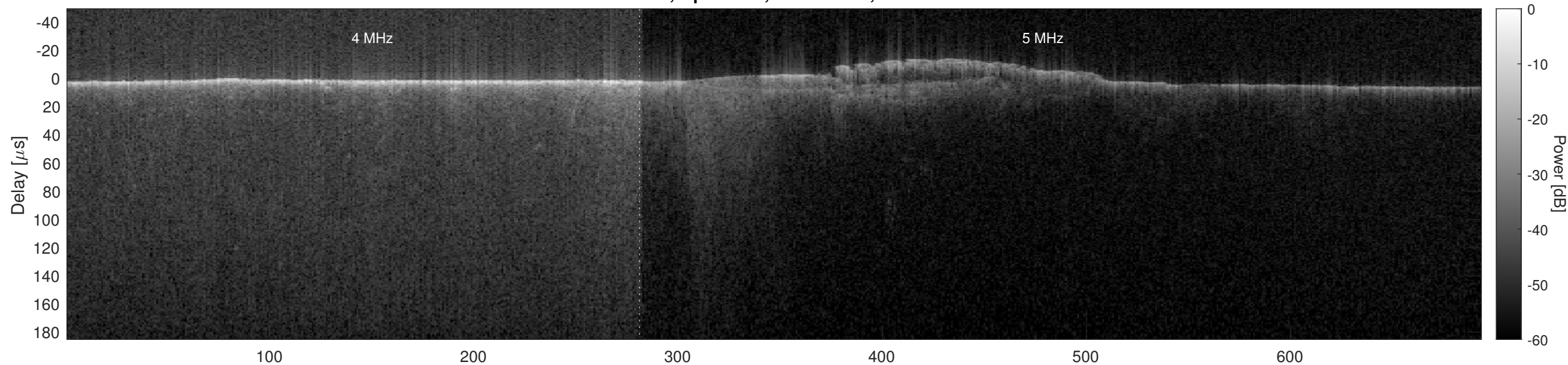
Orbit 7665, Optimized, No Window, Channel 2
