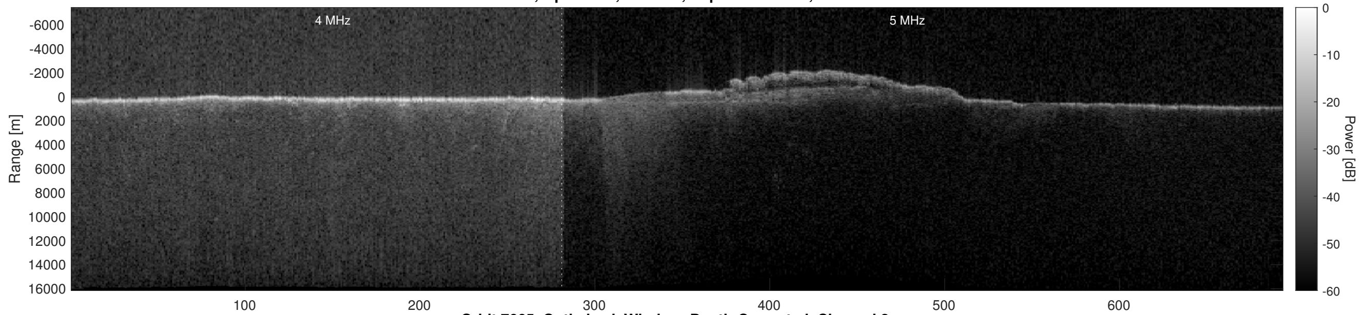
Orbit 7665, Optimized, Window, Depth-Corrected, Channel 2
