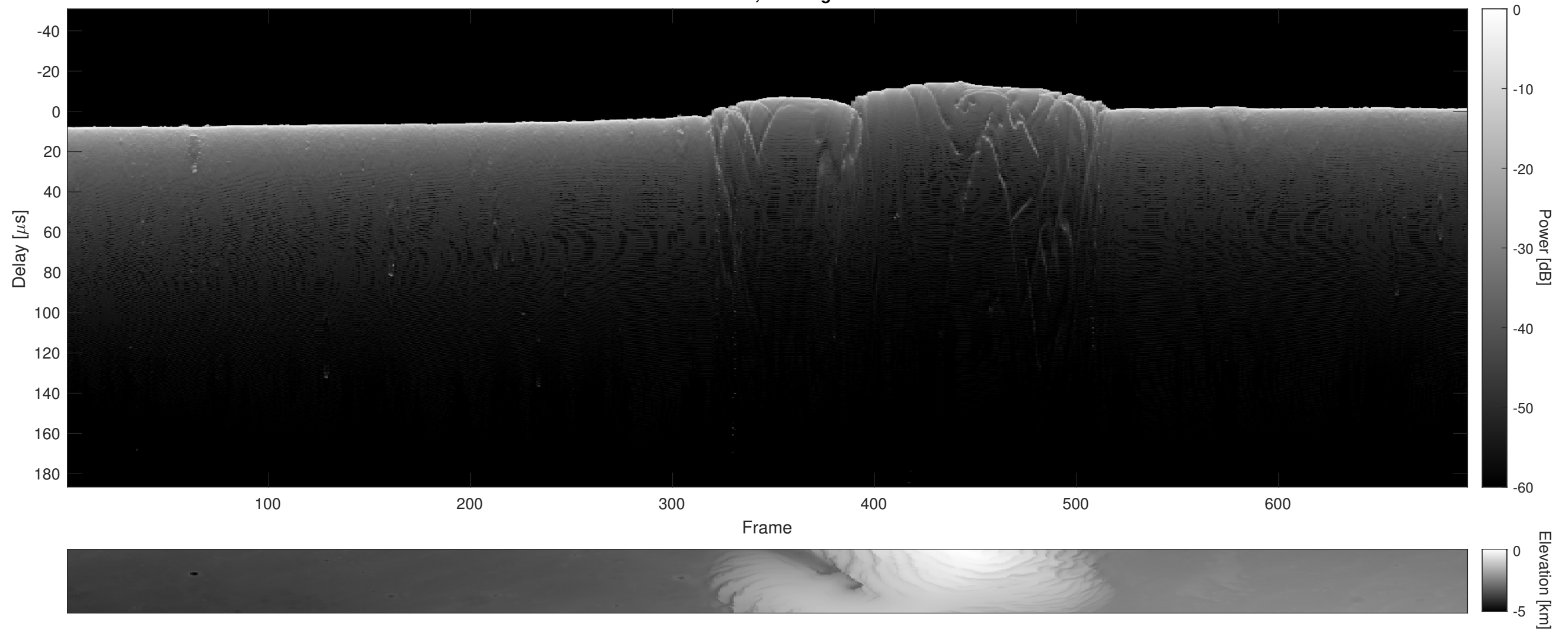
Orbit 7674, Cluttergram
