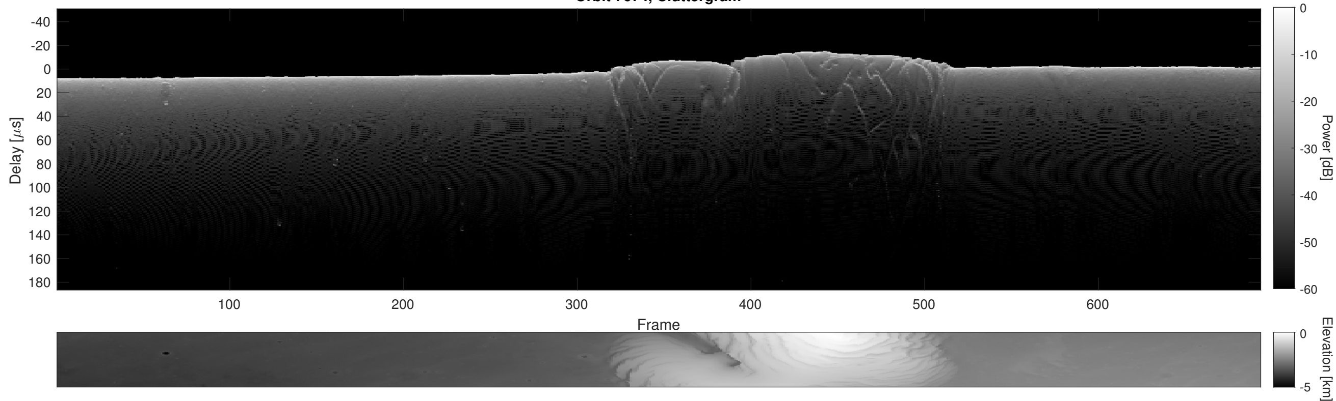
Orbit 7674, Cluttergram
