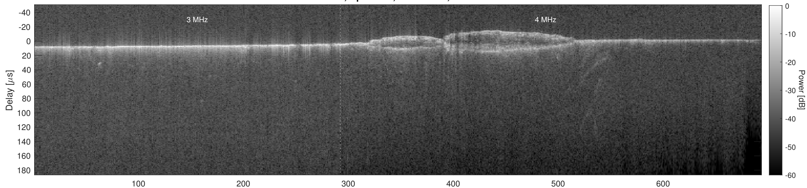
Orbit 7674, Cluttergram
