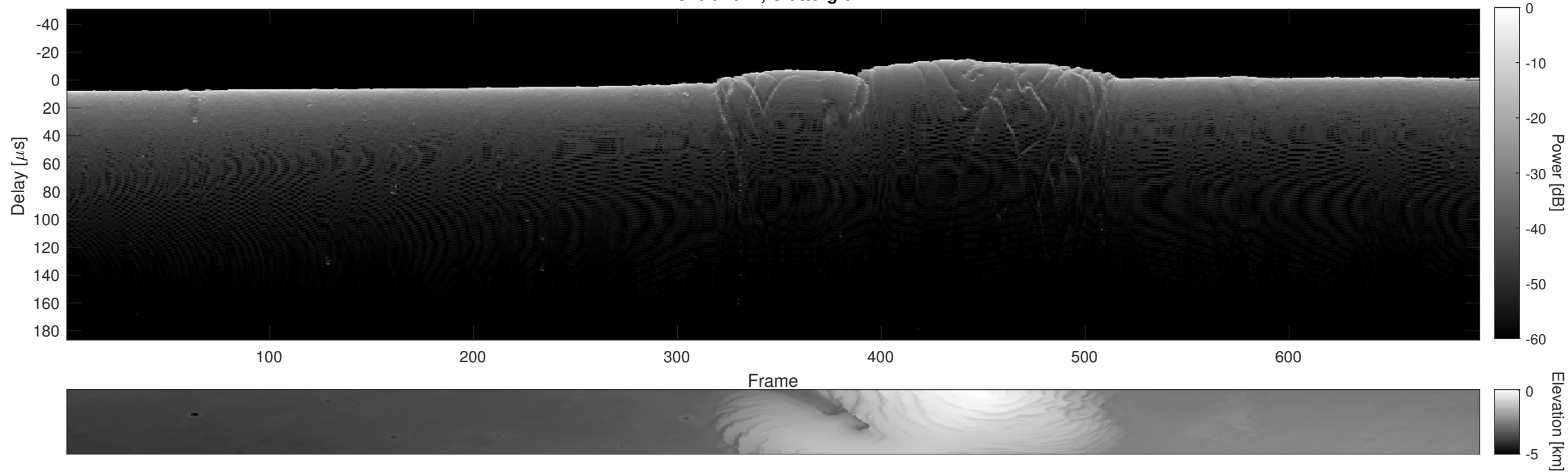
Orbit 7674, Cluttergram
