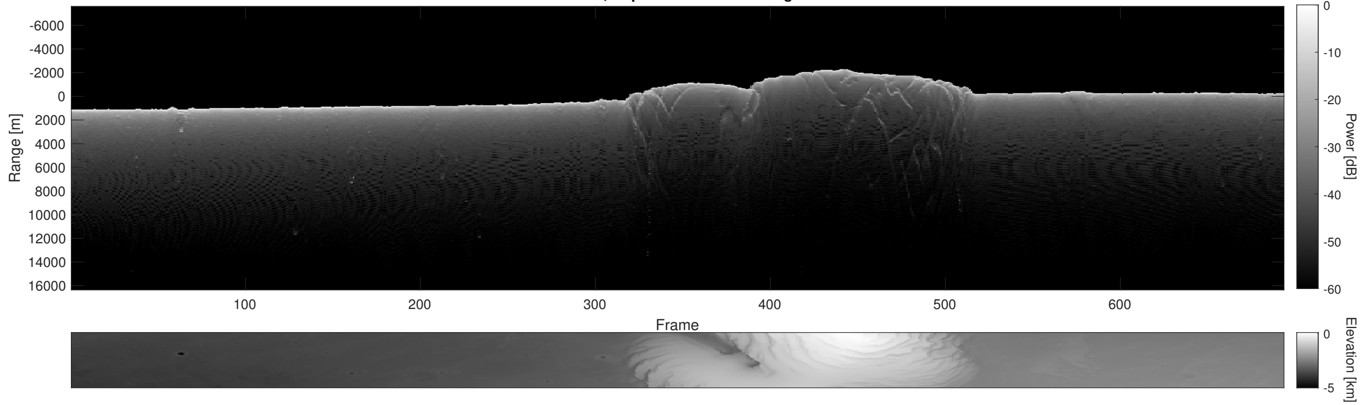
Orbit 7674, Depth-Corrected Cluttergram
