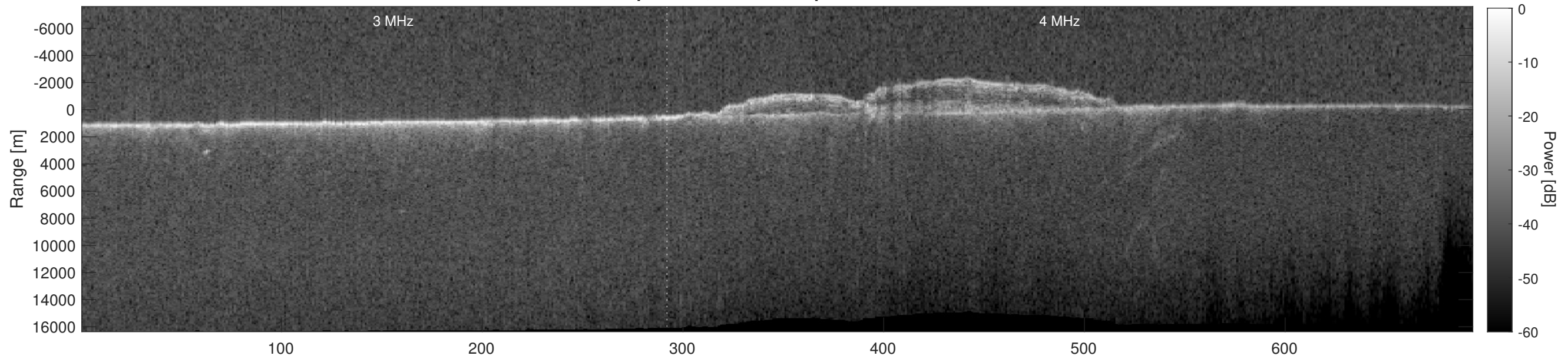
Orbit 7674, Depth-Corrected Cluttergram
