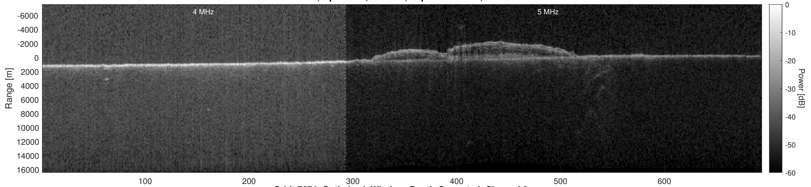
Orbit 7674, Optimized, Window, Depth-Corrected, Channel 2
