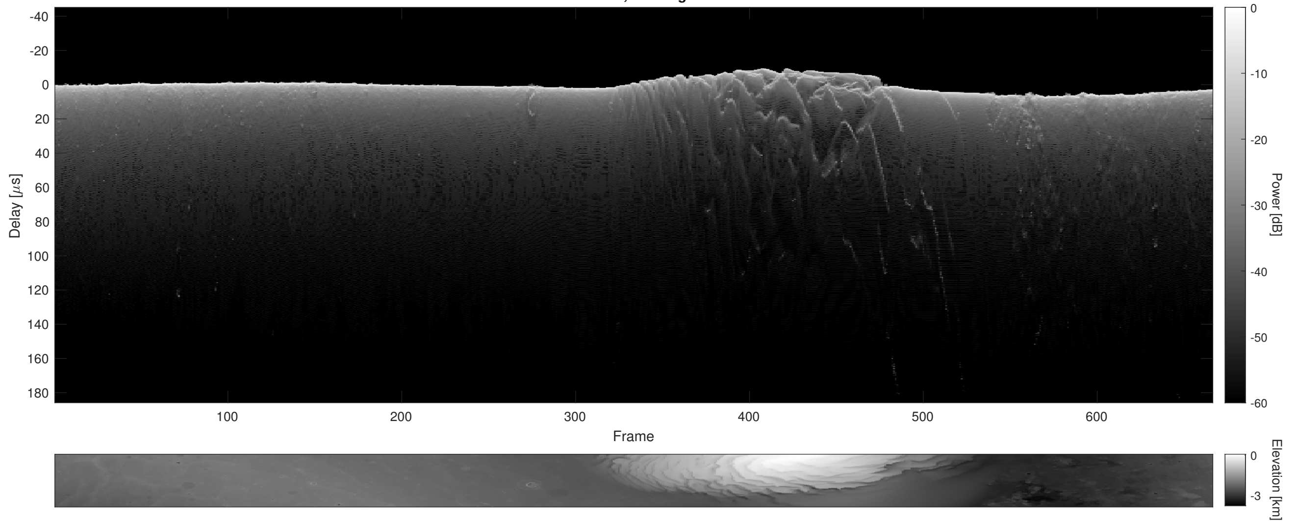
Orbit 7680, Cluttergram
