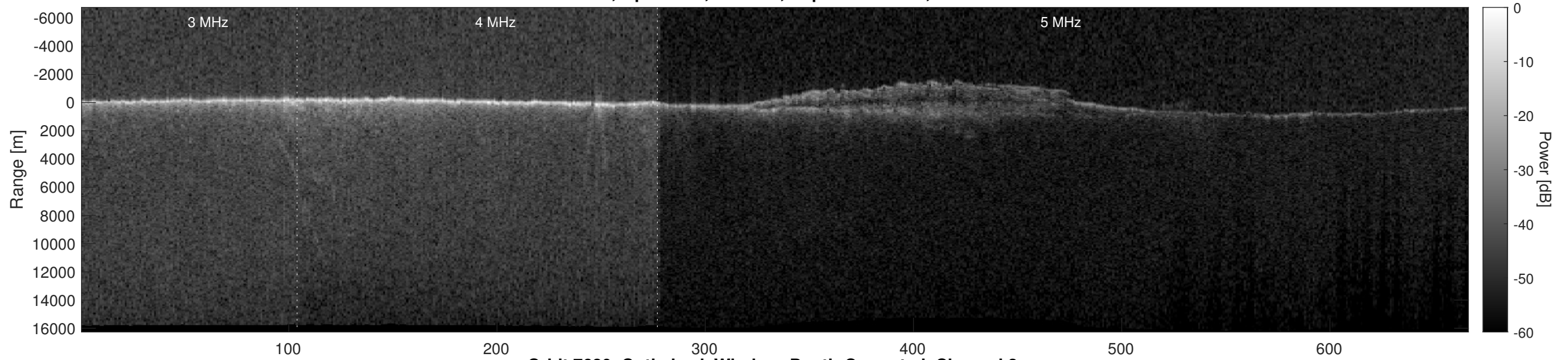
Orbit 7680, Optimized, Window, Depth-Corrected, Channel 2
