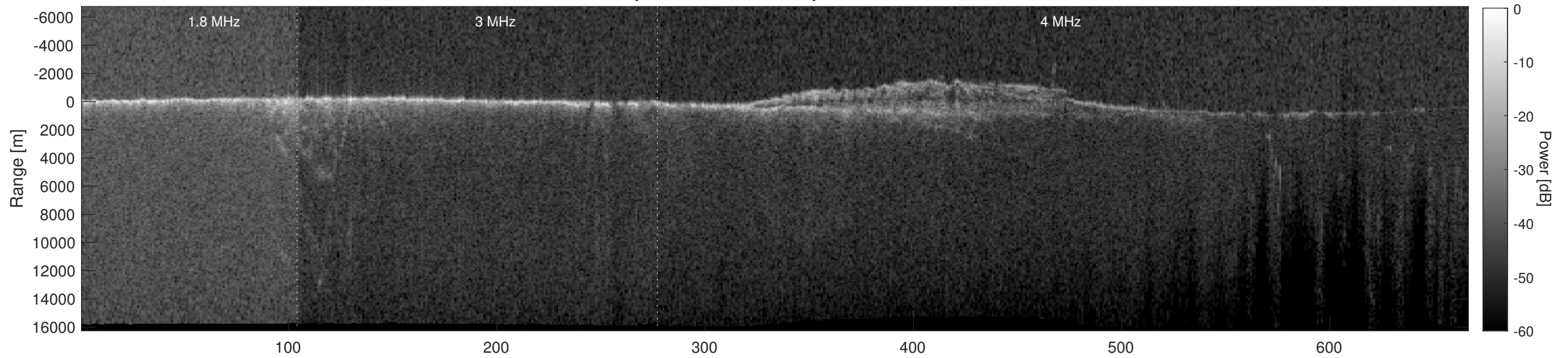
Orbit 7680, Depth-Corrected Cluttergram
