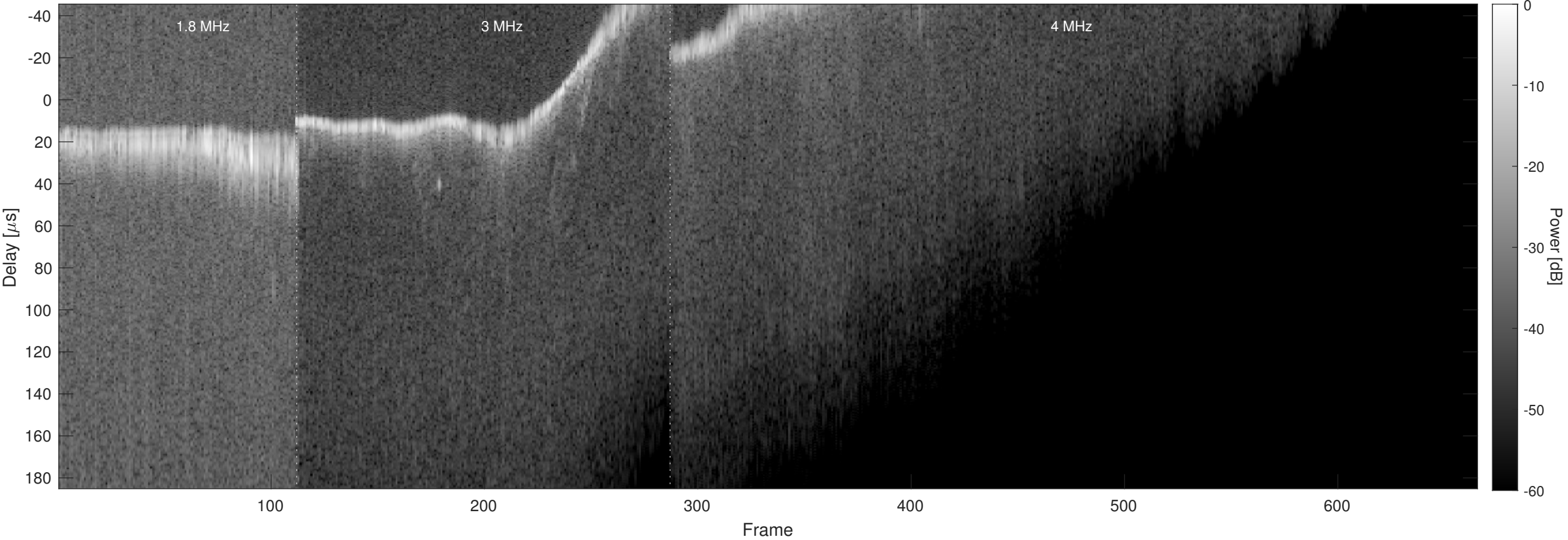
Orbit 7687, Chapman, Window, Channel 2
