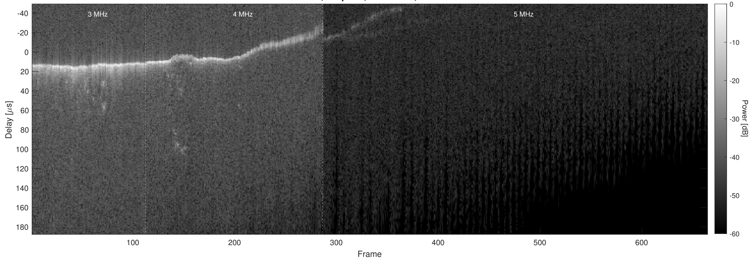
Orbit 7688, Chapman, No Window, Channel 2
