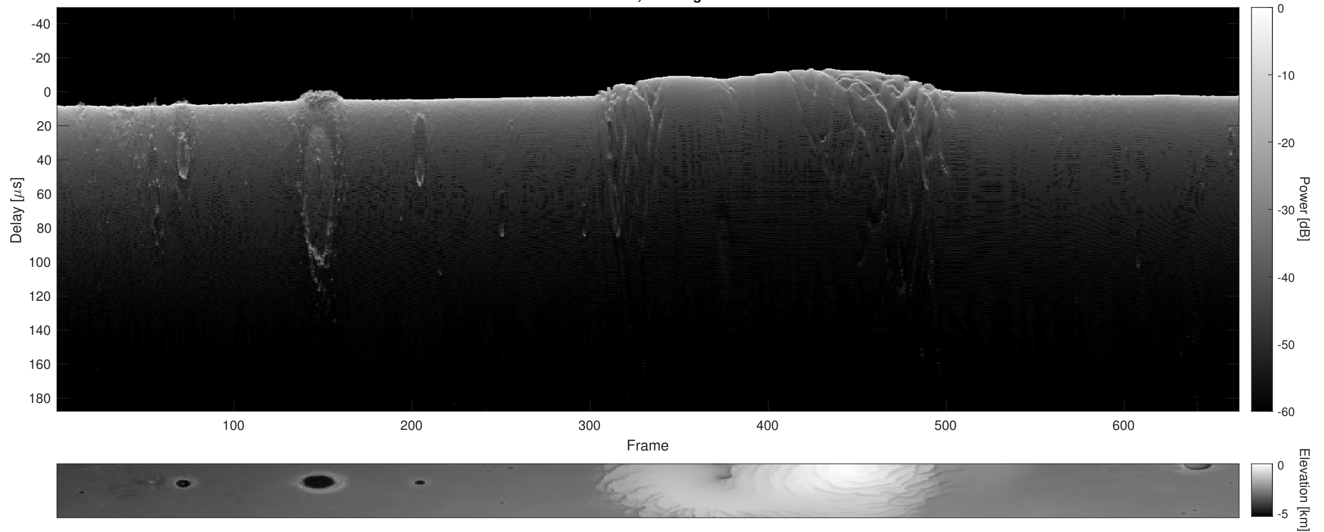
Orbit 7688, Cluttergram
