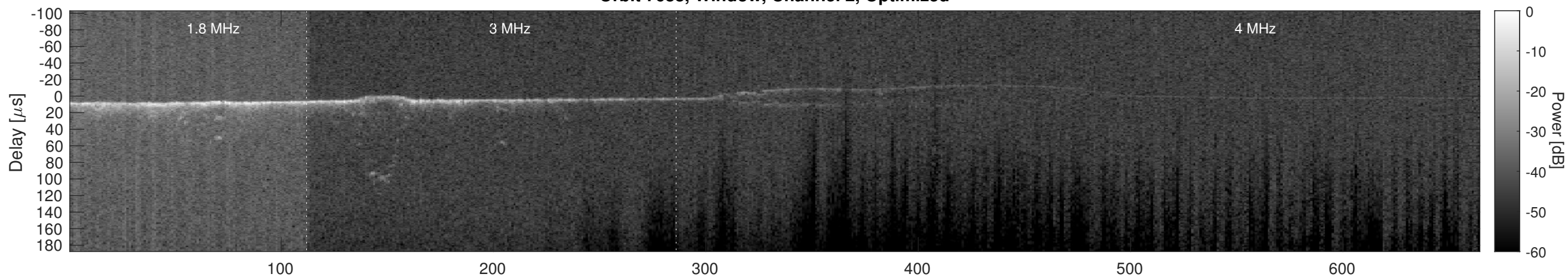
Orbit 7688, Cluttergram
