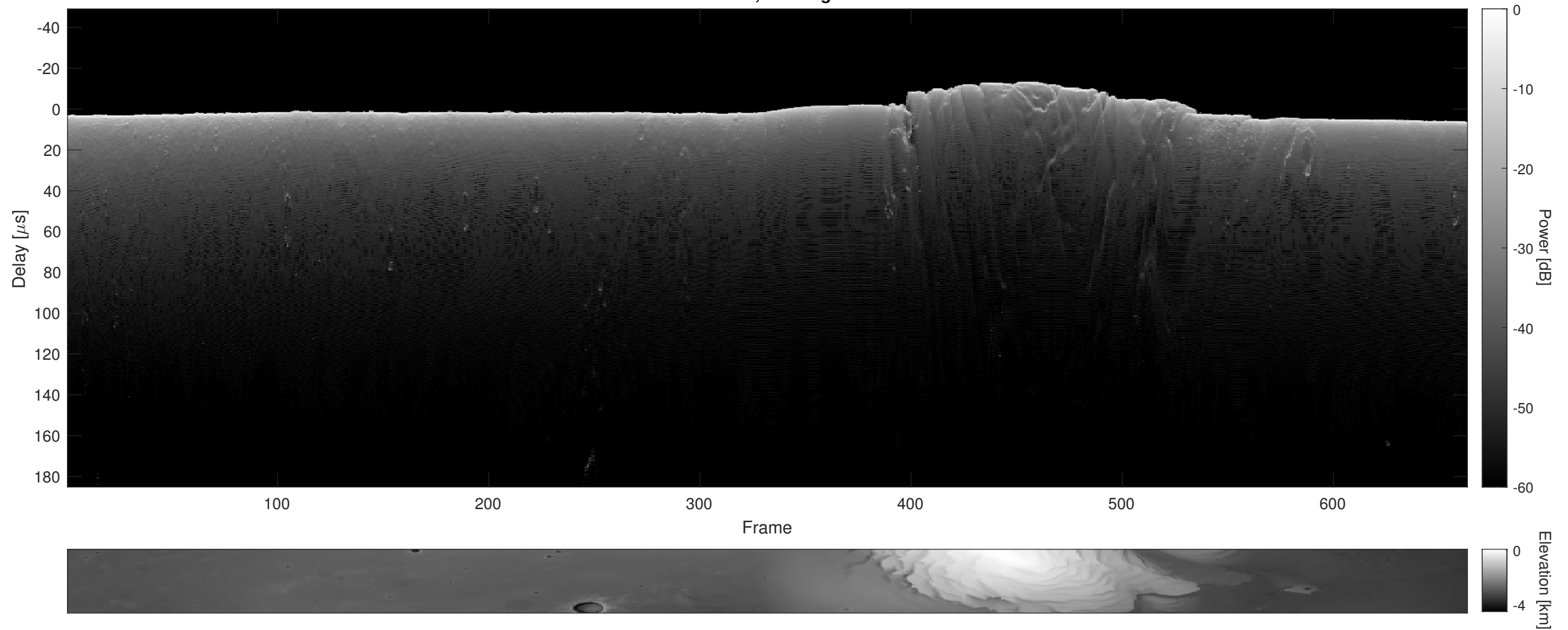
Orbit 7690, Cluttergram
