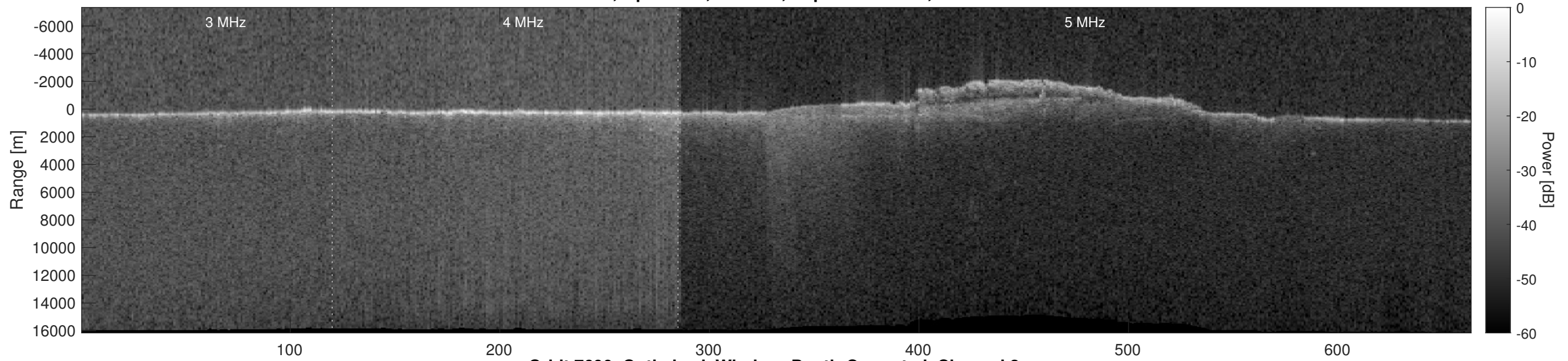
Orbit 7690, Optimized, Window, Depth-Corrected, Channel 2
