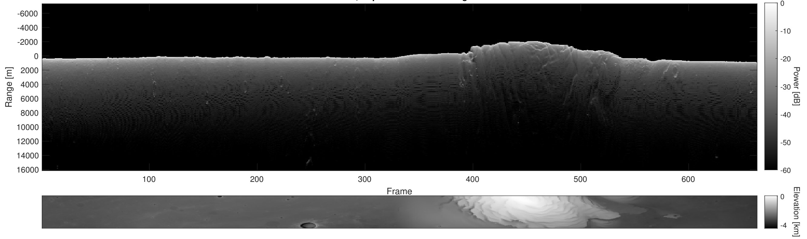
Orbit 7690, Depth-Corrected Cluttergram
