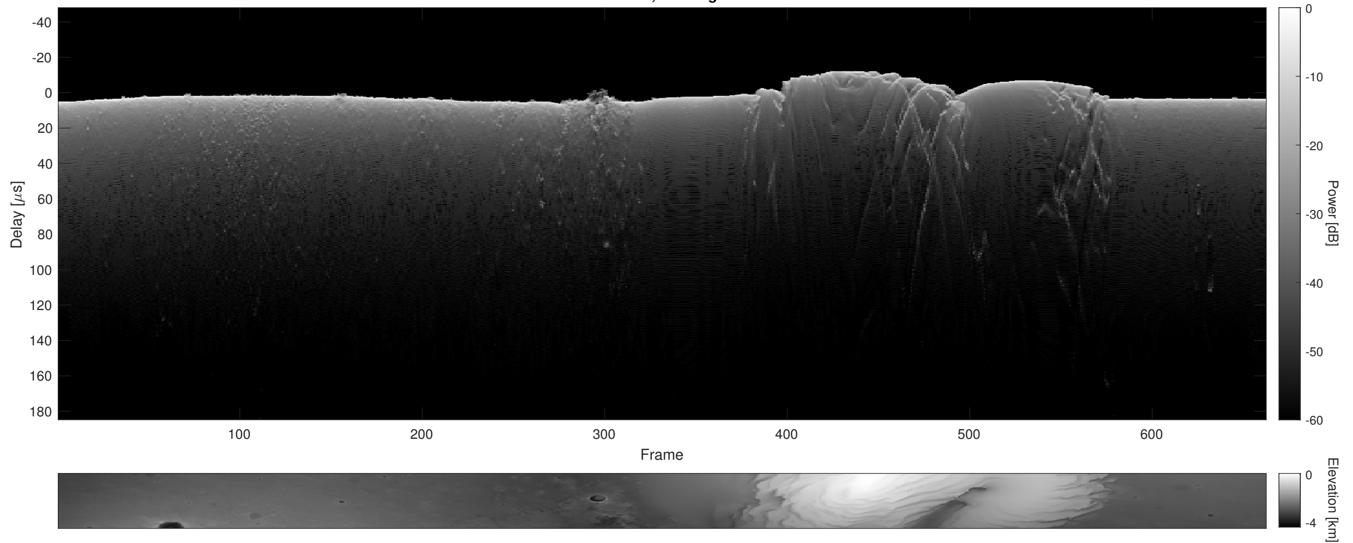
Orbit 7693, Cluttergram
