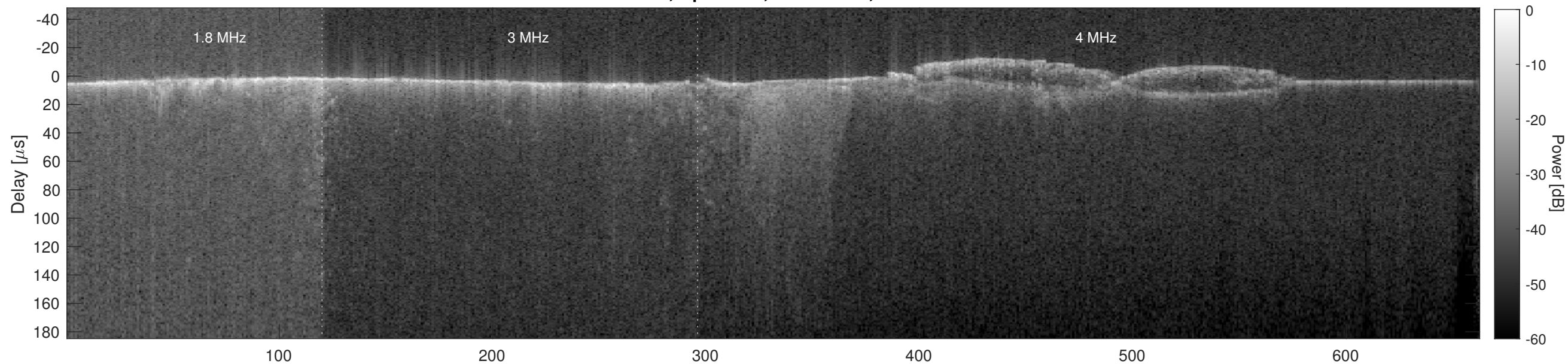
Orbit 7693, Cluttergram
