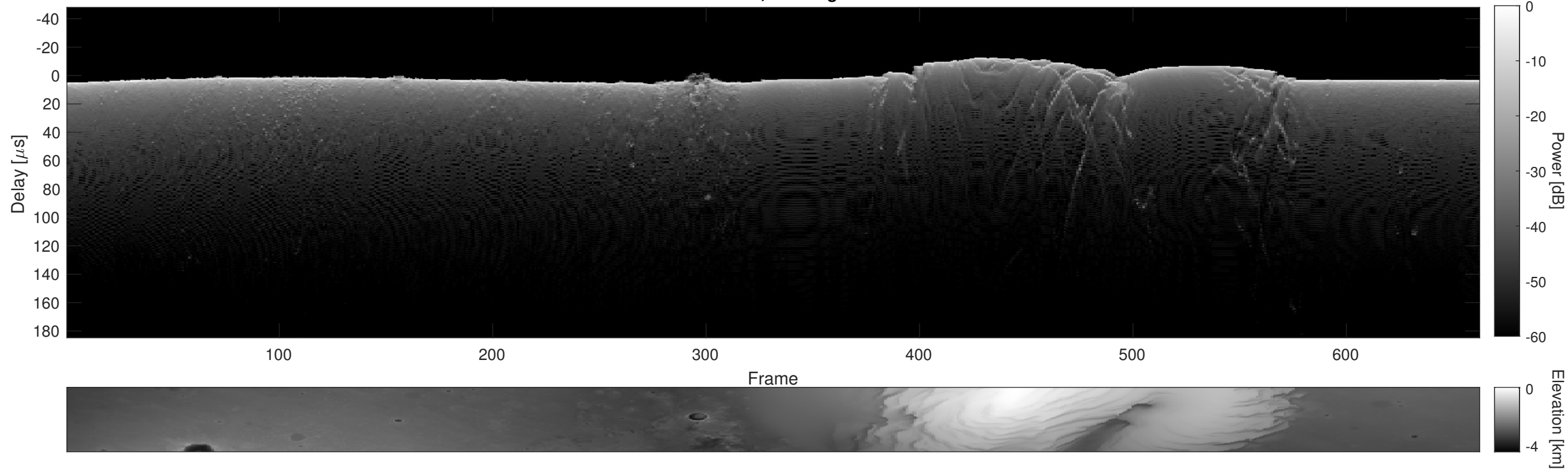
Orbit 7693, Cluttergram
