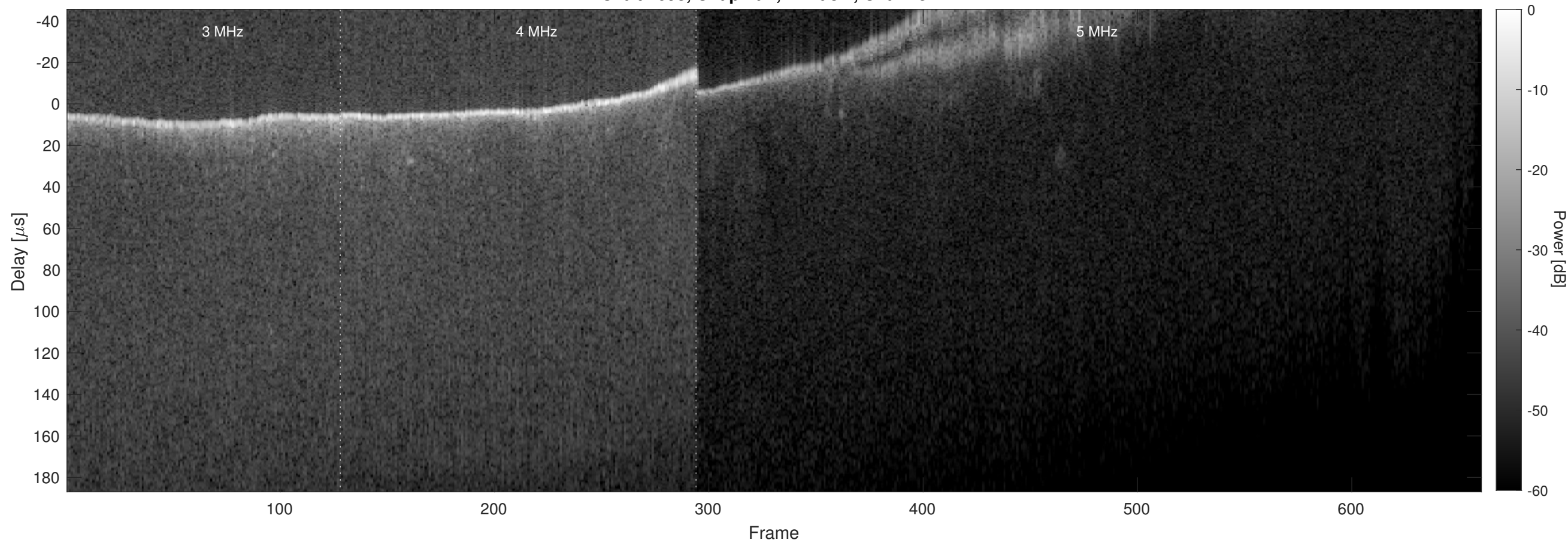
Orbit 7698, Chapman, Window, Channel 2
