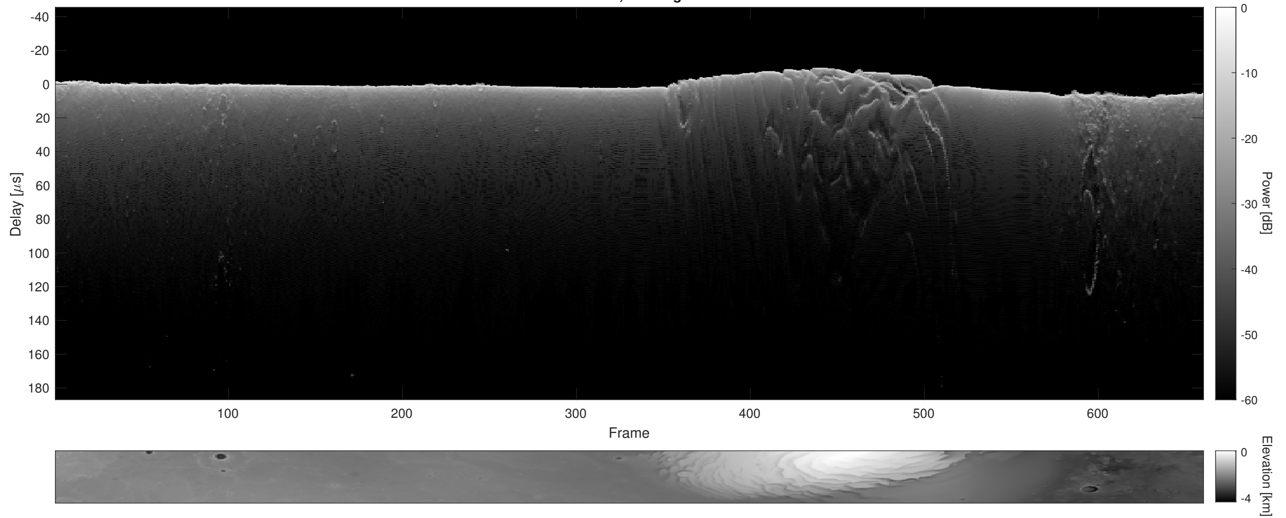
Orbit 7698, Cluttergram
