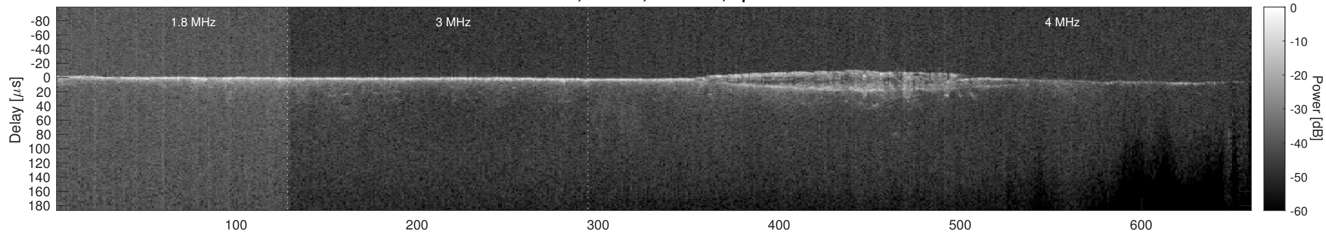
Orbit 7698, Cluttergram
