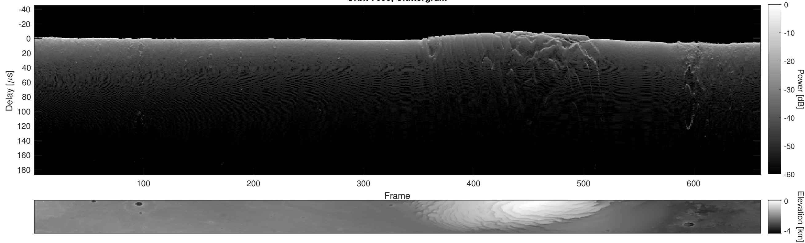
Orbit 7698, Cluttergram
