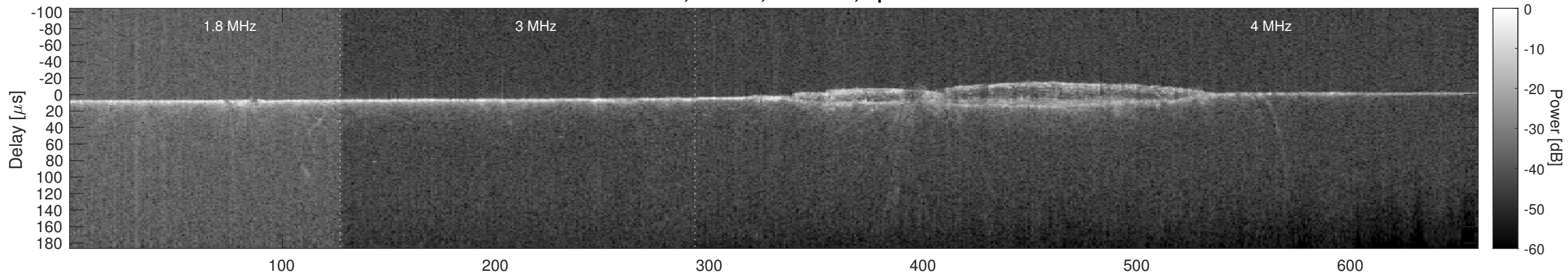
Orbit 7699, Cluttergram
